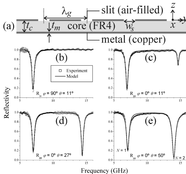
FIG. 1. Experimental reflectivity spectra and the numerically modeled results from the structure illustrated schematically in (a). (b) The R_{ss} response of the structure when orientated with the slit direction parallel to the plane of incidence ( \varphi = 90^\circ ). (c)–(e) The R_{pp} response with \varphi = 0^\circ at three different angles of incidence. The change in noise at 10 GHz corresponds to a switch in the set of waveguides and horn antennas used.
