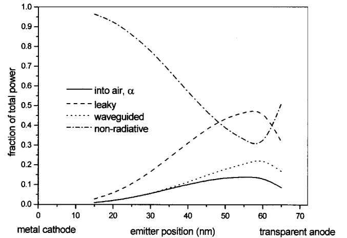
FIG. 9. The variation of \alpha and the contributions to the total power lost by a singlet exciton, as a function of emitter position in the polymer layer.
