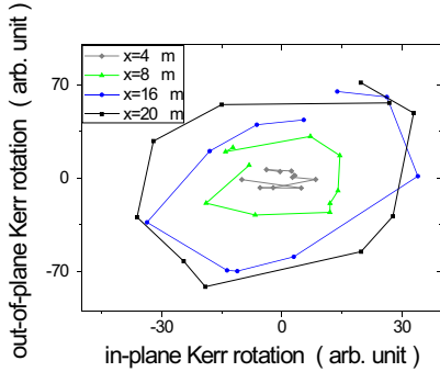
Fig. 5. Orbit of the 8 GHz mode at different positions ( x = 4, 8, 16, 20 \mu\text{m} ; y = 20 \mu\text{m} ).
