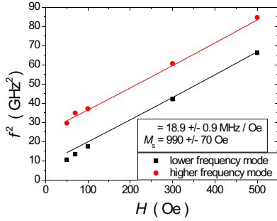
Fig. 8. Frequencies of the two modes vs. applied field. Fitting of this data with a Damon-Eshbach model yields M_s=990\pm 70 Oe and \gamma=18.9\pm 0.9 MHz/Oe for mode numbers n = 1, 3 .
