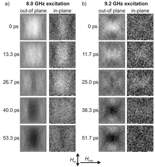
Fig. 3. Time-resolved images of the two modes at 500 Oe bias field. The sample was pumped with a sinusoidal magnetic field at 8.0 GHz (a) and 9.2 GHz (b), respectively. For both modes the out-of-plane component and the in-plane component perpendicular to the static magnetization direction are shown.
