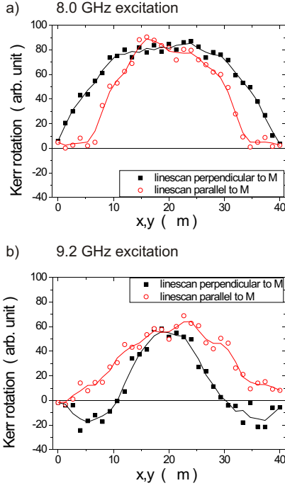
Fig. 4. Linescan through the center of the out-of-plane image of the 8.0 GHz mode (a) and 9.2 GHz mode (b) at 0 ps. There is a clear change of sign visible for the dynamic magnetization of the 9.2 GHz mode along the y-axis. The lines are a 3 point average of the data points. The same scaling of the data has been applied throughout the paper.
