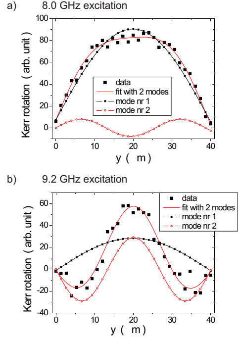
Fig. 6. Linescan across the out-of-plane image of the 8.0 GHz mode (a) and 9.2 GHz mode (b) at 0 ps and a fit using sine functions with two different wavelengths. The individual sine curves determined from the fit are also displayed.
