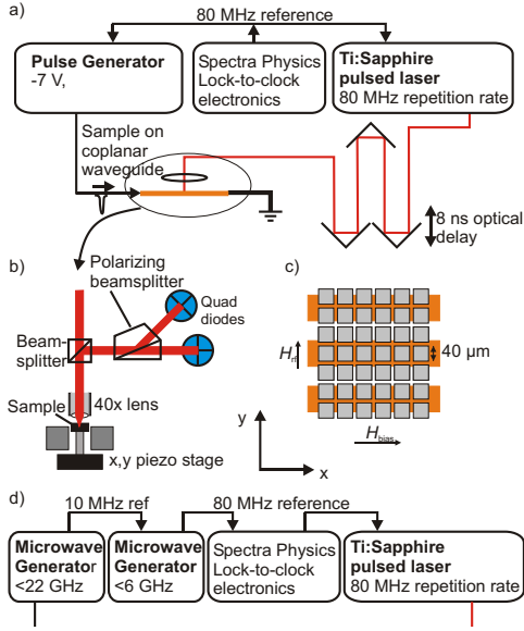
Fig. 1. (a) Experimental setup showing the laser system, synchronizing clock, optical delay line, and pulse generator. The optical detection of the Kerr rotation is shown in (b). The sample is placed face-down on a coplanar waveguide (c). For the harmonic excitation the pulse generator is replaced by a microwave generator and a second microwave generator is needed to phase lock the first microwave generator to the laser.
