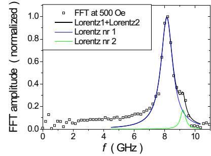
Fig. 7. Fit of the spectrum at 500 Oe to two Lorentzian functions.
