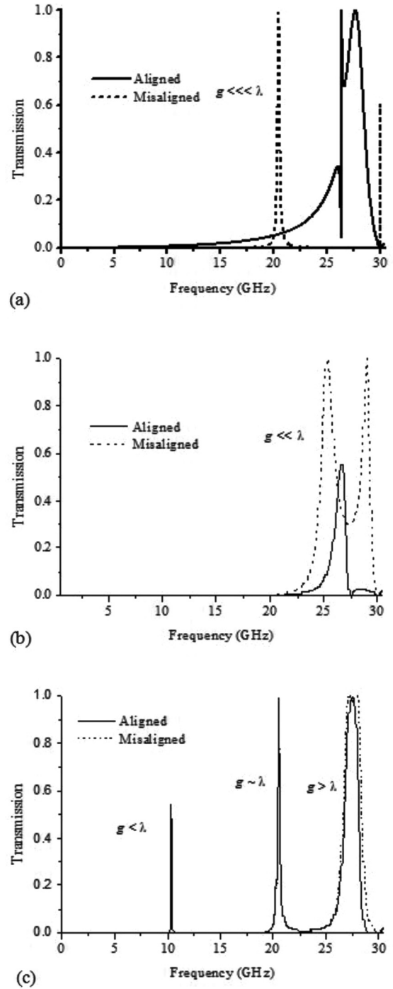
FIG. 2. Transmission for d = 10 mm, a = 4.5 mm for (a) g = 0.1 mm, (b) g = 4 mm, and (c) g = 14 mm. Each graph shows the results for both the aligned system and when the meshes are misaligned by 5 mm with respect to each other.
