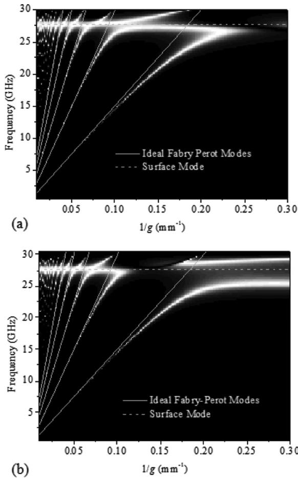
FIG. 3. Gray-scale plot of normal incidence transmission as a function of frequency and mesh separation with pitch 10 mm and hole sides 4.5 mm for (a) b = 0 mm and (b) b = 5 mm. The ideal Fabry-Pérot modes refer to the half-wavelength condition (i.e., \lambda = 2d/n for n = 1, 2, 3, \dots ).
