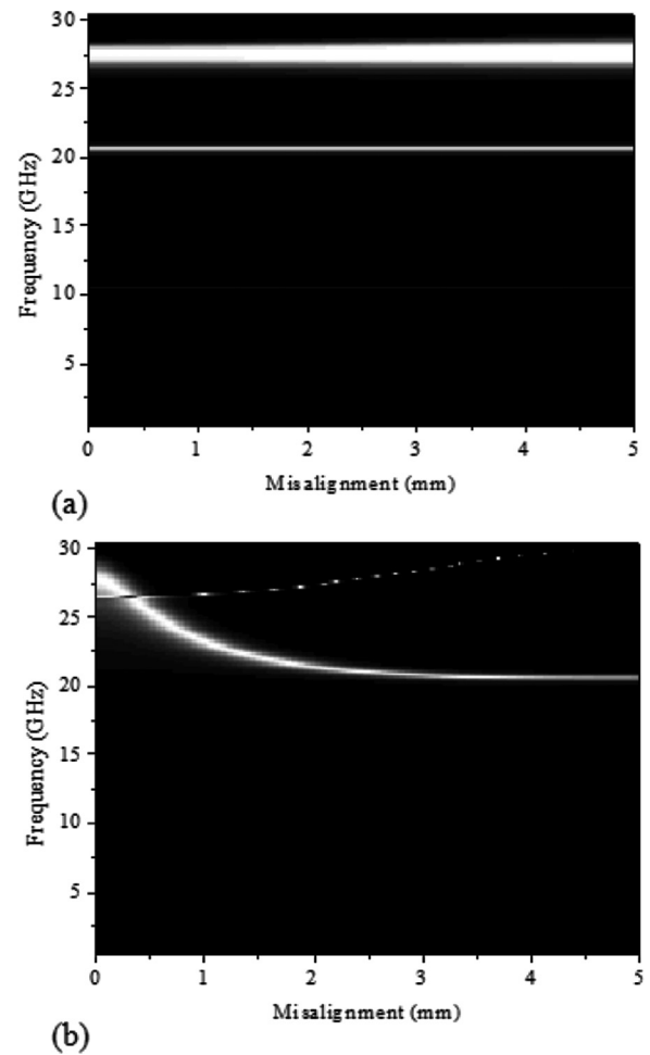
FIG. 4. Gray-scale plot of normal incidence transmission as a function of frequency and misalignment with pitch 10 mm and hole sides 4.5 mm for (a) mesh separation 14 mm and (b) mesh separation 0.1 mm.
