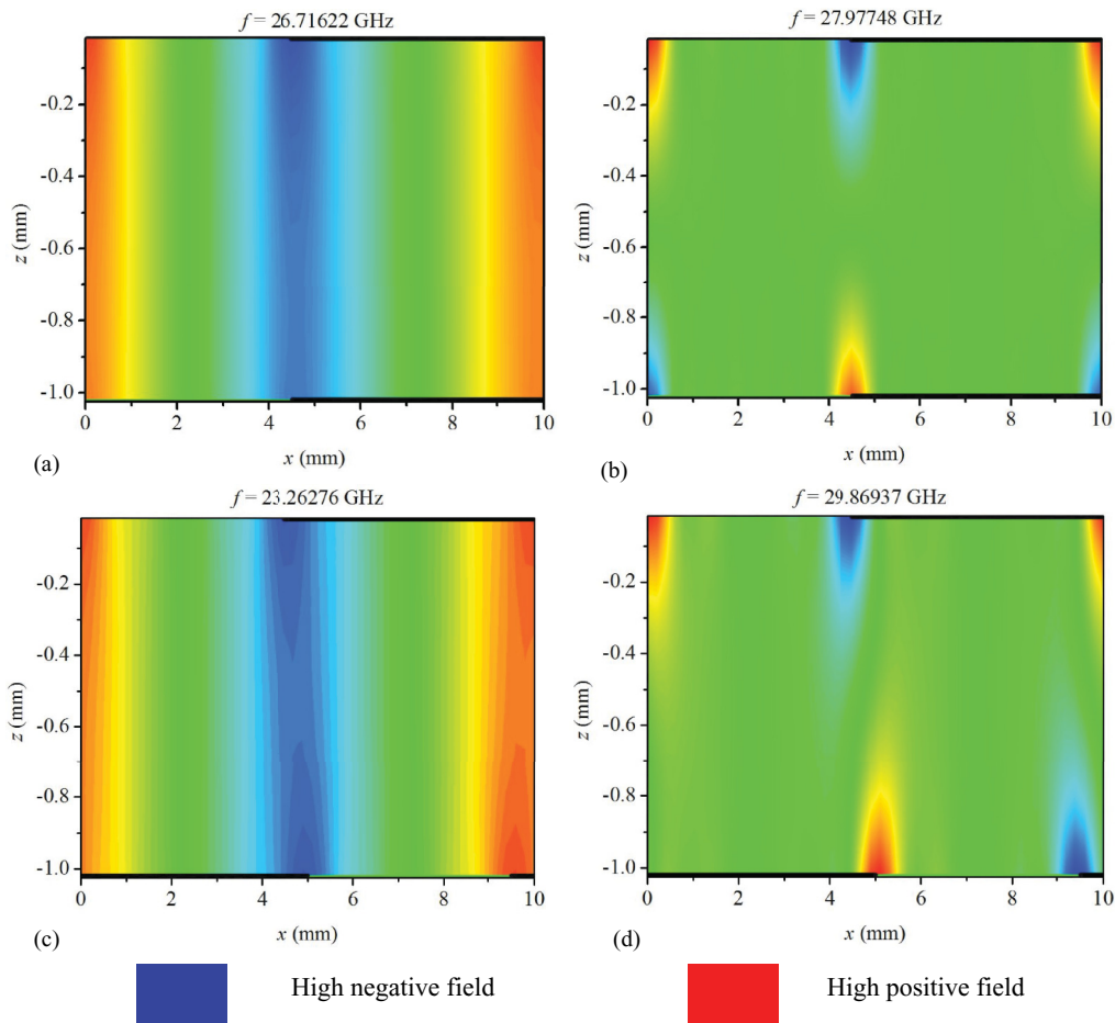
FIG. 7. (Color online) Directional E field plots in the XZ plane in the region between the two meshes for a double-mesh-layer system of pitch d = 10 mm, hole side length a = 4.5 mm, and mesh separation g = 1 mm at (a) 26.7 GHz with misalignment b = 0 mm; (b) 28.0 GHz with misalignment b = 0 mm; (c) 23.3 GHz with misalignment b = 5 mm; and (d) 29.9 GHz with misalignment b = 5 mm. The metal meshes are represented by thick black lines.
