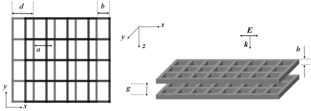
FIG. 1. Schematic of the investigated geometry; 2D square array of square holes (unshaded) in a PEC sheet (shaded).
