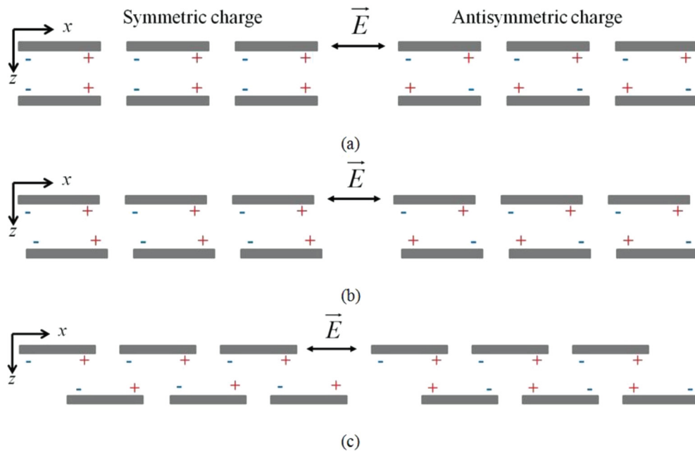
FIG. 6. (Color online) Schematic of possible charge distributions for a double layer of identical metal slit arrays (one-dimensional grids) when the layers are (a) aligned with respect to each other; (b) slightly misaligned with respect to each other, and (c) at maximum misalignment with respect to each other.
