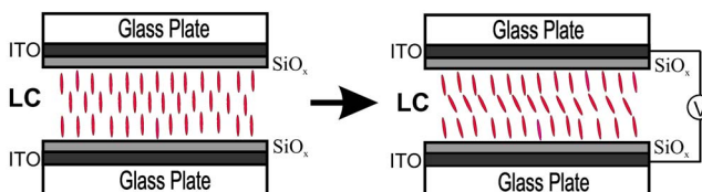
FIG. 2. (Color online) Schematic of the cell structure and the change of the director orientation after applying an electric field.
