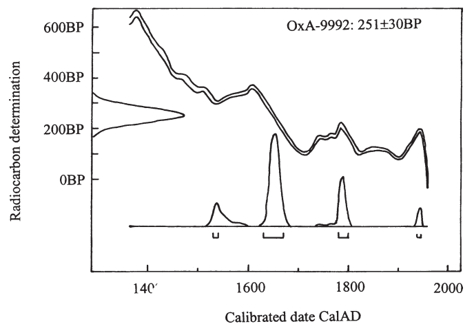
Figure 6. AMS dating results showing the most likely age for Godrevy dog to be between 1620 and 1680 AD.
