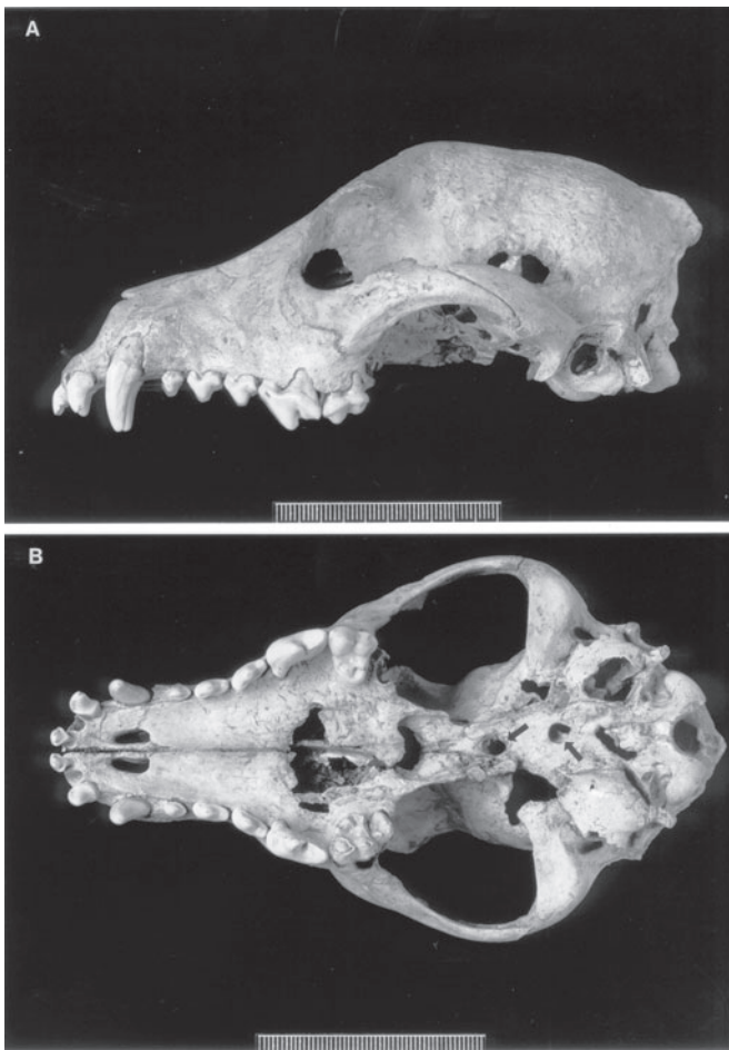
Figure 5. Photographs showing the skull of Godrevy dog. (a) Side profile of the skull; note that the dentition is fully erupted. (b) View of the underside of the skull. Note the two small apertures in the region of the basi-sphenoid bone (arrowed). These are smooth sided and appear to be pathological in origin. Scale bar in both photographs is in mm.
