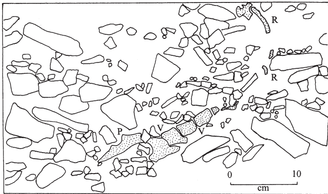
Figure 3. Schematic diagram showing the field appearance of the skeletal remains weathering from the cliff section at Godrevy prior to excavation. The skeletal remains were enclosed within coarse clasts of vein quartz and Devonian metasediments in a poorly sorted clayey matrix. P - pelvis, V - vertebrae, R - rib.
