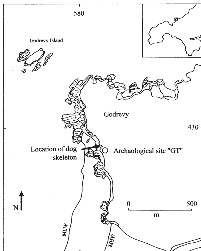
Figure 1. Map showing the location of the studied section at Godrevy. The approximate location of Mesolithic and Romano-British sites in the area is also indicated (based upon Thomas, 1958).
