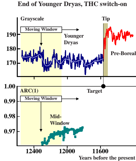
Fig. 14. A second illustration taken from Dakos et al. [2008] for the end of the Younger Dryas event using the grayscale from basin sediment in Cariaco, Venezuela. The whole of the above ARC(1) graph fits in the red circle of Figure 4.
