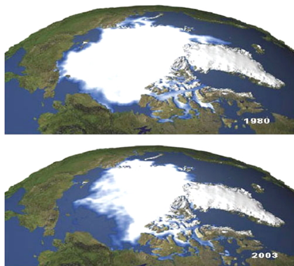
Fig. 3. Two NASA satellite photographs, showing the reduction of Arctic snow and ice cover over a 23 year interval. Source: http://nasascience.nasa.gov/images/about-us/accomplishments/YIR2004_arctic.jpg
