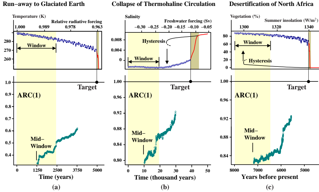
Fig. 12. Results of Dakos et al. [2008] for three examples based on predictive models. (a) Run-away to glaciated Earth ( N = 800 ), (b) Collapse of thermohaline circulation ( N = 1000 ), (c) Desertification of North Africa ( N = 6002 ). Notice the notional hysteresis loops sketched on (b) and (c). These pictures have been re-drawn as mid-window plots.
