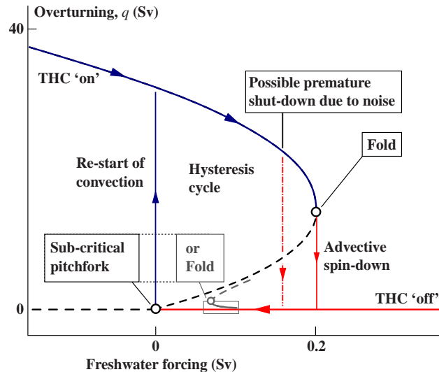
Fig. 10. A schematic diagram of the thermohaline response showing the two bifurcations and the associated hysteresis cycle [Rahmstorf, 2000]. The subcritical pitchfork bifurcation will be observed in very simple models, but will be replaced by a fold in more elaborate ones: see, for example, Figure 12(b). Note that 1Sv is 10^6 cubic metres per second, which is roughly the combined flow rate of all rivers on Earth.
