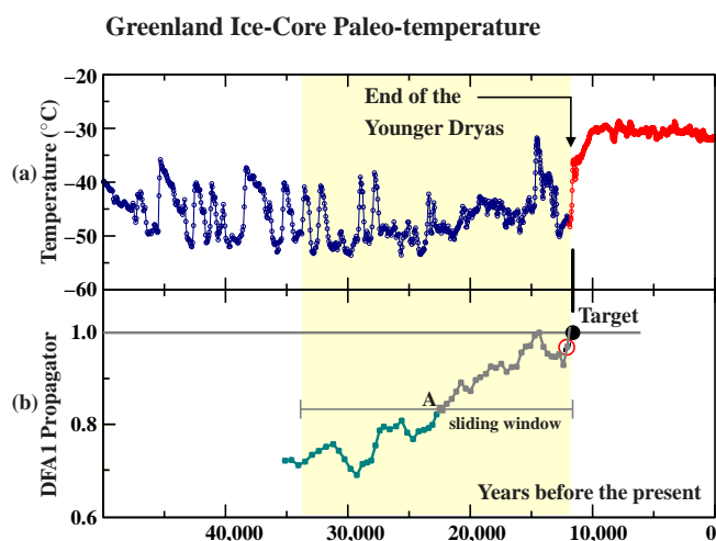
Fig. 4. Results of Livina & Lenton [2007] for the end of the last glaciation (a) Greenland ice-core (GISP2) paleo-temperature with an unevenly spaced record, visible in the varying density of symbols on the curve. The total number of data points is N = 1586 . In (b) the DFA1-propagator is calculated in sliding windows of length 500 points and mapped into the middle points of the windows. The results of a second and much more local study by Dakos et al. [2008] (that we shall be discussing in Figure 14) are highlighted by the red circle.
