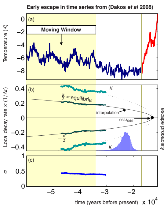
Fig. 7. Estimated probability for early escape from the stable node based on the AR(1) analysis of the ice-core record from the end of the last glaciation [Petit et al. , 1999]. Figure (a) shows the original time series, (b) the estimated local decay rate per time step, \kappa , the corresponding equilibrium positions for the saddle-node normal form, and the interpolation estimate for the critical time t_{\text{fold}} . The inset in (b) shows the probability distribution for escape. Figure (c) shows the estimate for the non-dimensionalized noise-level.
