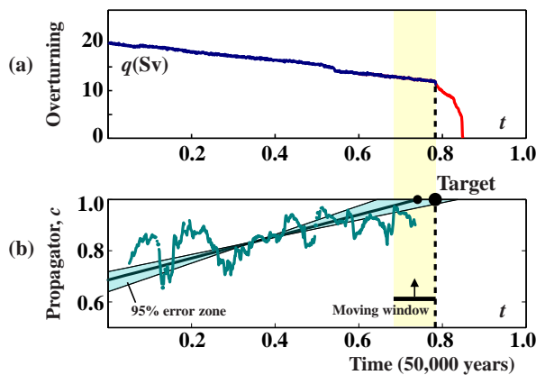
Fig. 11. Results of [Held & Kleinen, 2004] which give a good prediction of the collapse of the thermohaline circulation induced by a 4-fold linear increase of CO 2 over 50,000 years in a model simulation. Collapse present at t \approx 0.8 in (a) is predicted to occur when the propagator, c = \text{ARC}(1) , shown in (b), or its linear fit, reaches +1.
