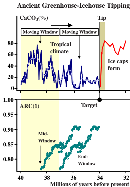
Fig. 13. The ancient greenhouse to icehouse tipping with N = 482 data points. This is one of the best correlations obtained by Dakos et al. [2008] in their work on eight recorded tipping points. Here the sediments containing \text{CaCO}_3 were laid down 30–40 million years ago. Re-drawn from Dakos et al. [2008], as described in the text.
