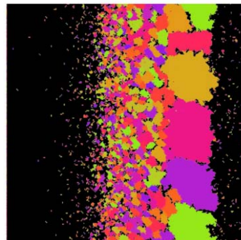
Fig. 2 Crystal structure in sample of \text{Ge}_2\text{Sb}_2\text{Te}_5 where the left boundary is held at 227^\circ\text{C} and the right at 477^\circ\text{C} for 23\ \mu\text{s} .
