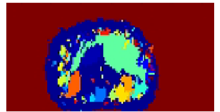
Fig. 3 The (partial) re-crystallization of the amorphous mushroom-shaped dome of a PCRAM cell. A fully crystallized cell was initially amorphized (reset) with a 1.5V, 40ns pulse. The figure shows the state of re-crystallization after the application 200ns after the application of a 0.8V set pulse.
