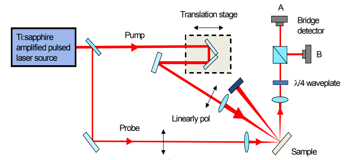
Fig. 8 Time-resolved laser set-up for femtosecond crystallization and amorphization experiments
