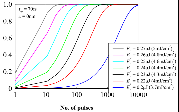
Fig. 10 Predicted fraction of crystallization of \text{Ge}_2\text{Sb}_2\text{Te}_5 optical disk sample subjected to multiple 70 fs pulses with energies in the range 0.2 \mu\text{J} to 0.27 \mu\text{J} .
