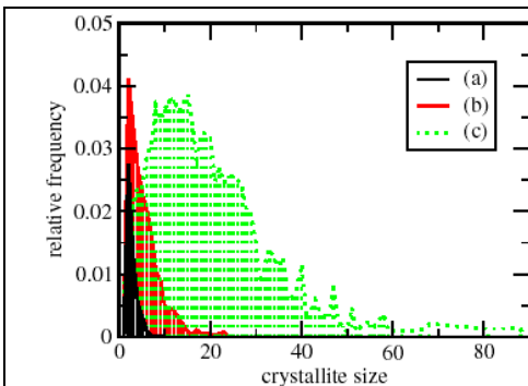
Fig. 1 Relative frequency of crystallites of different sizes for a \text{Ge}_2\text{Sb}_2\text{Te}_5 sample bulk annealed at 131^\circ\text{C} for (a) 248s (b) 743s and (c) 68,930 s. There is a peak in the crystal size distribution of 10-15 nm for the fully developed crystal structure.
