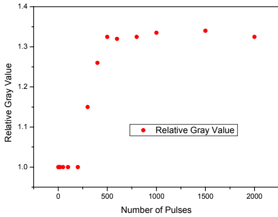
Fig. 9 Experimental results for crystallization of \text{Ge}_2\text{Sb}_2\text{Te}_5 optical disk sample using multiple 0.2 \mu\text{J} femtosecond pulses. The sample remains in the pre-switching 'energy accumulation' mode until around 250 pulses are received in this case.
