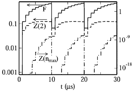
Fig. 7 Simulated fraction of crystallized material (F) and concentration of dimers ( Z(2) ) and multimers ( Z(n_{\max}) ) for a series of nine 350°C, 50 ns excitation pulses. The phase-change cell accumulates energy and crystal fraction with each pulse and re-amorphized after the ninth pulse.
