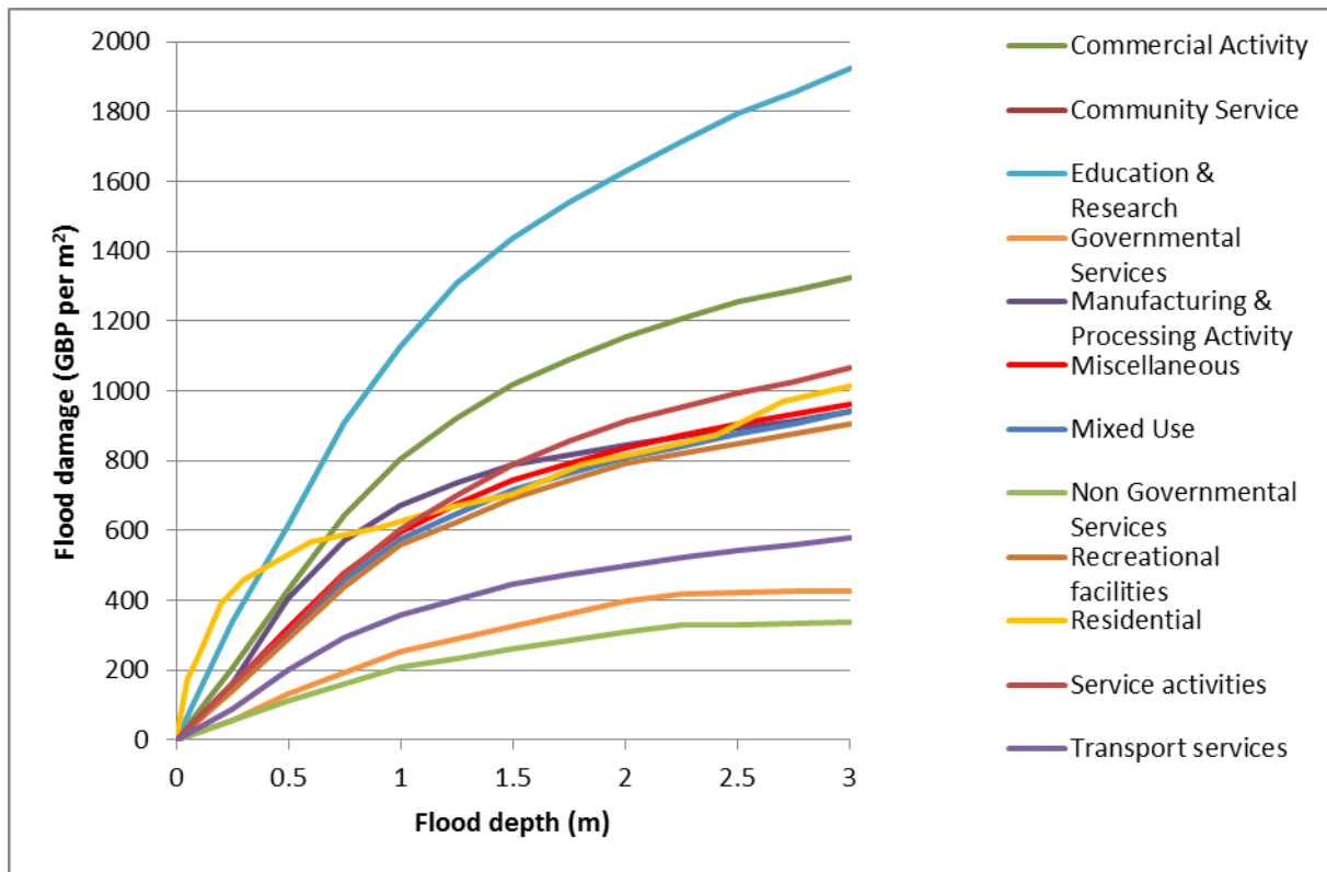
Figure 2 - Flood depth - damage functions
