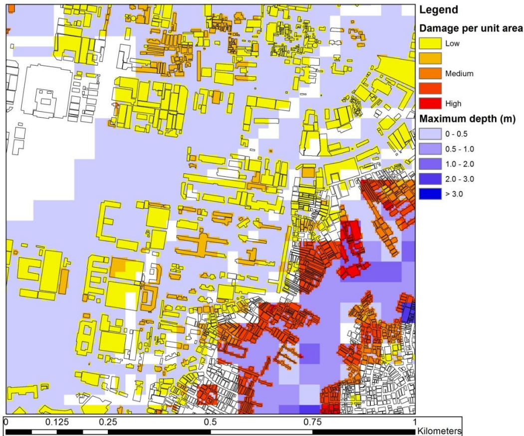
Figure 5 - Building damage per unit area
