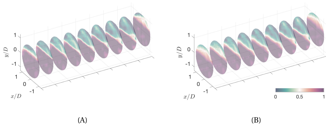
Figure 5.6: (A) Full order instantaneous phase fraction tomograms and (B) reduced order instantaneous phase fraction tomograms of slug flow, reconstructed with 3 eigenmodes. The reduced order dynamical description includes prominent flow features using three degrees of freedom. The full order description of the flow uses 1250 degrees of freedom.
