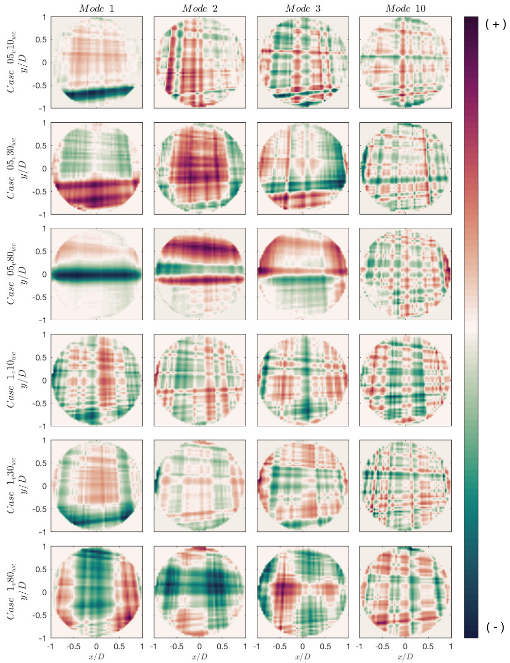
Figure 4.3: Eigenmodes 1, 2, 3 and 10 for all cases. The modes show the most dominant structures of the flow with respect to spatial location. The most important structures are present in the first mode.
