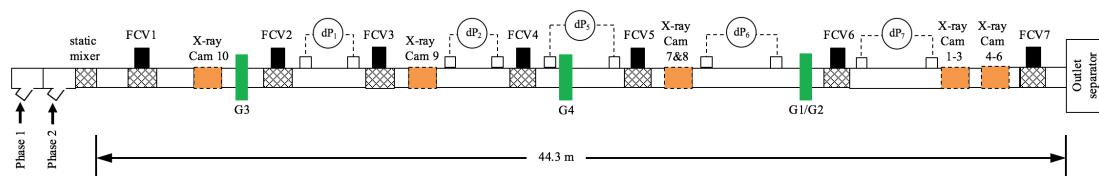
Figure 3.1: Experimental test section (not to scale).
