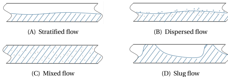
Figure 1.1: Side view of two-phase flow for visualization of dynamics for various multiphase regimes.
