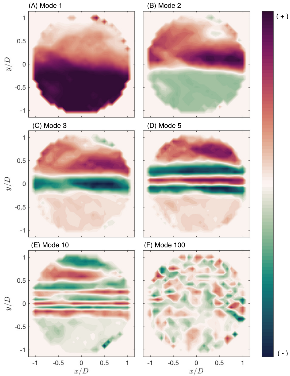
Figure 5.4: Eigenmodes 1, 2, 3, 5, 10 and 100 for the slug flow case depicted in (A) through (F), respectively. The first mode shows the mean phase fraction of the slug flow with successive modes depicting the main features of the flow spatially.
