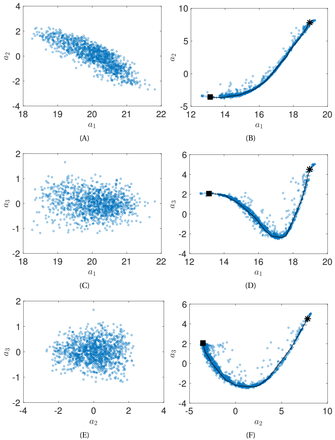
Figure 5.7: Phase correlation diagrams of temporal coefficients for i = 1, 2 & 3 for dispersed flow (left column) and slug flow (right column). The asterisk and the square, included in the figures of slug flow, represent the formation at t = t_o and break up at t = t_f of the slug, respectively.
