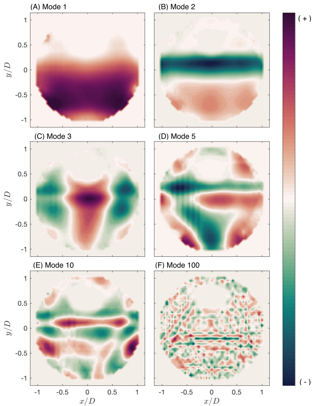
Figure 5.3: Eigenmodes 1, 2, 3, 5, 10 and 100 for the dispersed case depicted in (A) through (F), respectively. The modes show the most dominant structures of the flow in the cross-section of the pipe. The kernel of the POD is the instantaneous phase fraction therefore the most prominent structure is the mean phase fraction, shown in the first mode.
