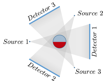
Figure 3.2: Orientation of source and detection devices for one X-ray system along the pipe.
