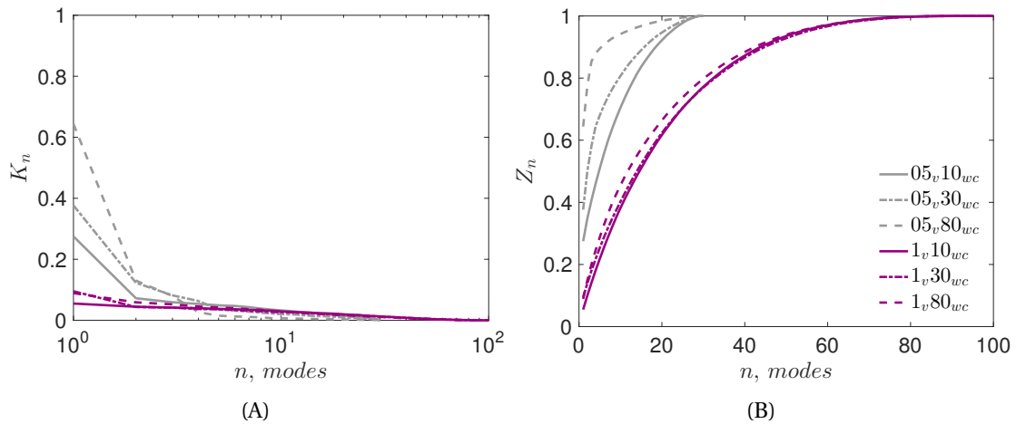
Figure 4.2: The distribution of variance described by (A) normalized eigenvalues, K_n , and (B) successive summation of eigenvalues, Z_n as a function of the mode, n . The value associated with each eigenvalues is representative of the amount of information present in the corresponding eigenmode.
