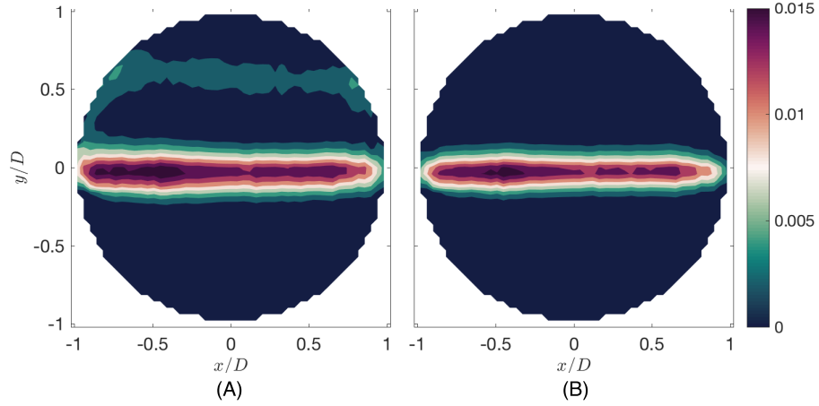
Figure 4.4: Phase fraction interactions, \langle \phi'_w \phi'_o \rangle , of 05_v 80_{wc} for full order description (left) and the 50% reconstructed reduced order description (right). The low order description shows the main features of the interaction between the two fluids. The reconstruction uses a single mode while the full order description requires all 30 degrees of freedom of the system.
