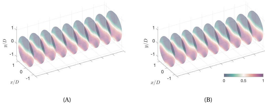
Figure 5.5: (A) Full order instantaneous phase fraction tomograms and (B) reduced order instantaneous phase fraction tomograms of dispersed flow, reconstructed with 1 eigenmode. The low order description shows main features of the flow while using less than 1% of the information from the full order model.
