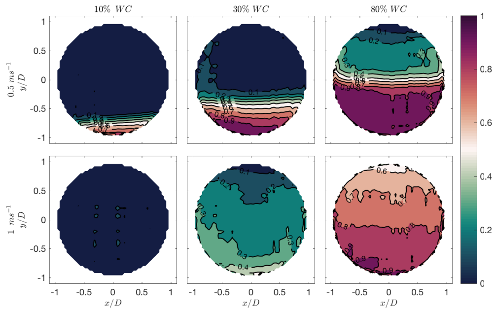
Figure 4.1: Time-averaged tomograms of the cross-sectional water distribution for stratified and mixed flow cases. The time-averaged tomograms show the most prominent characteristics of the flow field. Contour lines indicate the local water fraction in steps of 0.1.
