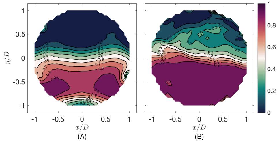
Figure 5.1: Mean phase fraction tomograms of the cross-sectional distribution (A) \langle \phi_w \rangle for dispersed flow and (B) \langle \phi_o \rangle for slug flow. Most prominent features of the phase fraction field are depicted. Contour lines indicate the local water fraction in steps of 0.1.
