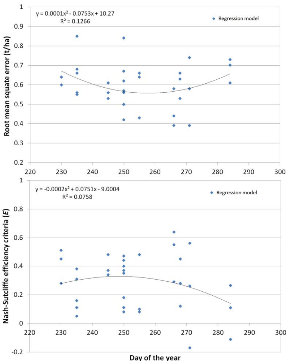
Figure 3. Root Mean Square Error (RMSE) and the Nash-Sutcliffe Efficiency Criteria ( E ) values by day of the year for the regression models.
