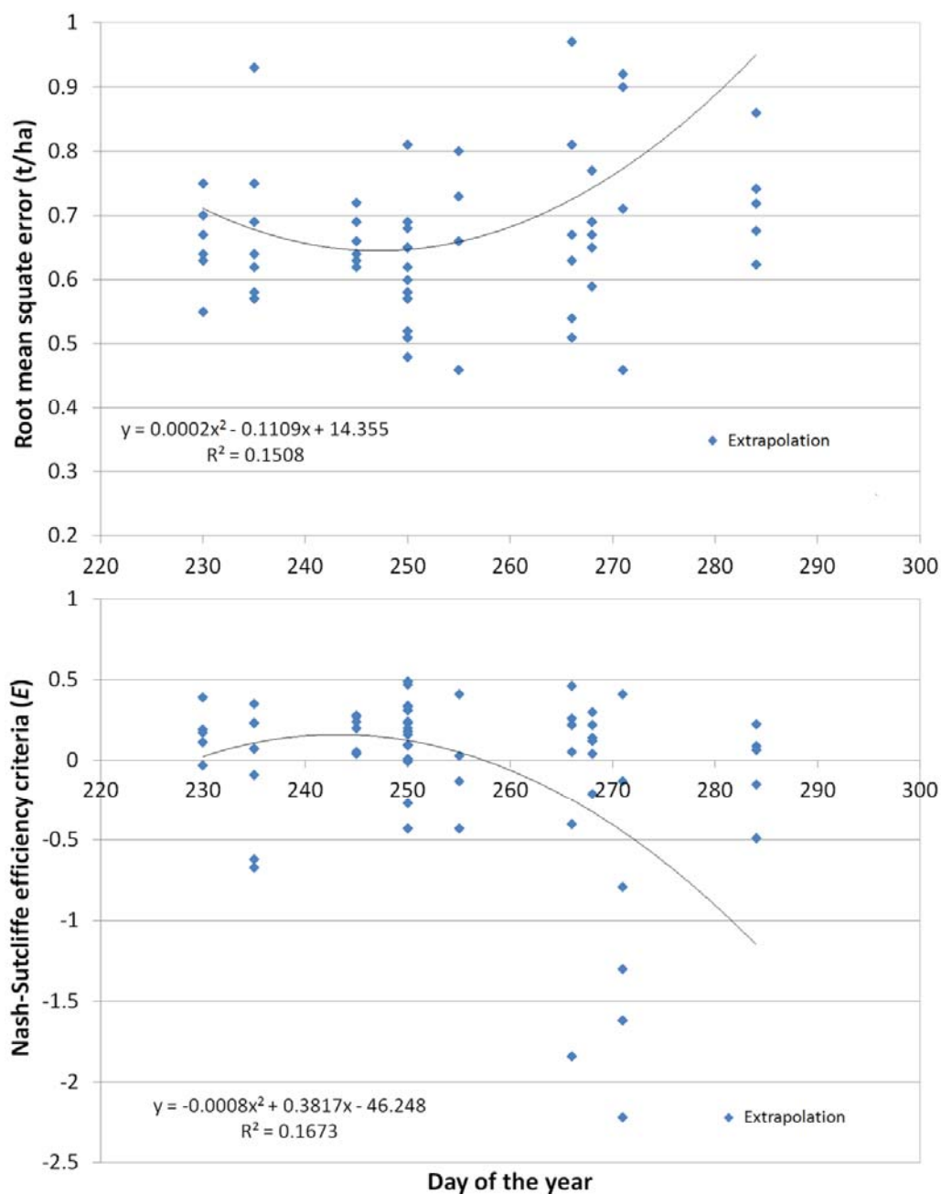
Figure 4. Root Mean Square Error (RMSE) and the Nash-Sutcliffe Efficiency Criteria ( E ) values by day of the year for the extrapolation of the regression models.
