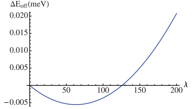
FIG. 2. (Color online) The energy shift \Delta E_{\text{off}} as a function of the parameter \lambda , using Eq. (43).
