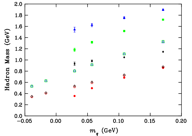
FIG. 7 (color online). Low-lying hadron mass spectrum obtained from the original configurations (full symbols) and the vortex-free configurations (open symbols). The symbols correspond to the various hadrons considered. For the original configurations, from lowest to highest hadron masses, the symbols correspond to \pi , \rho , N and \Delta .
