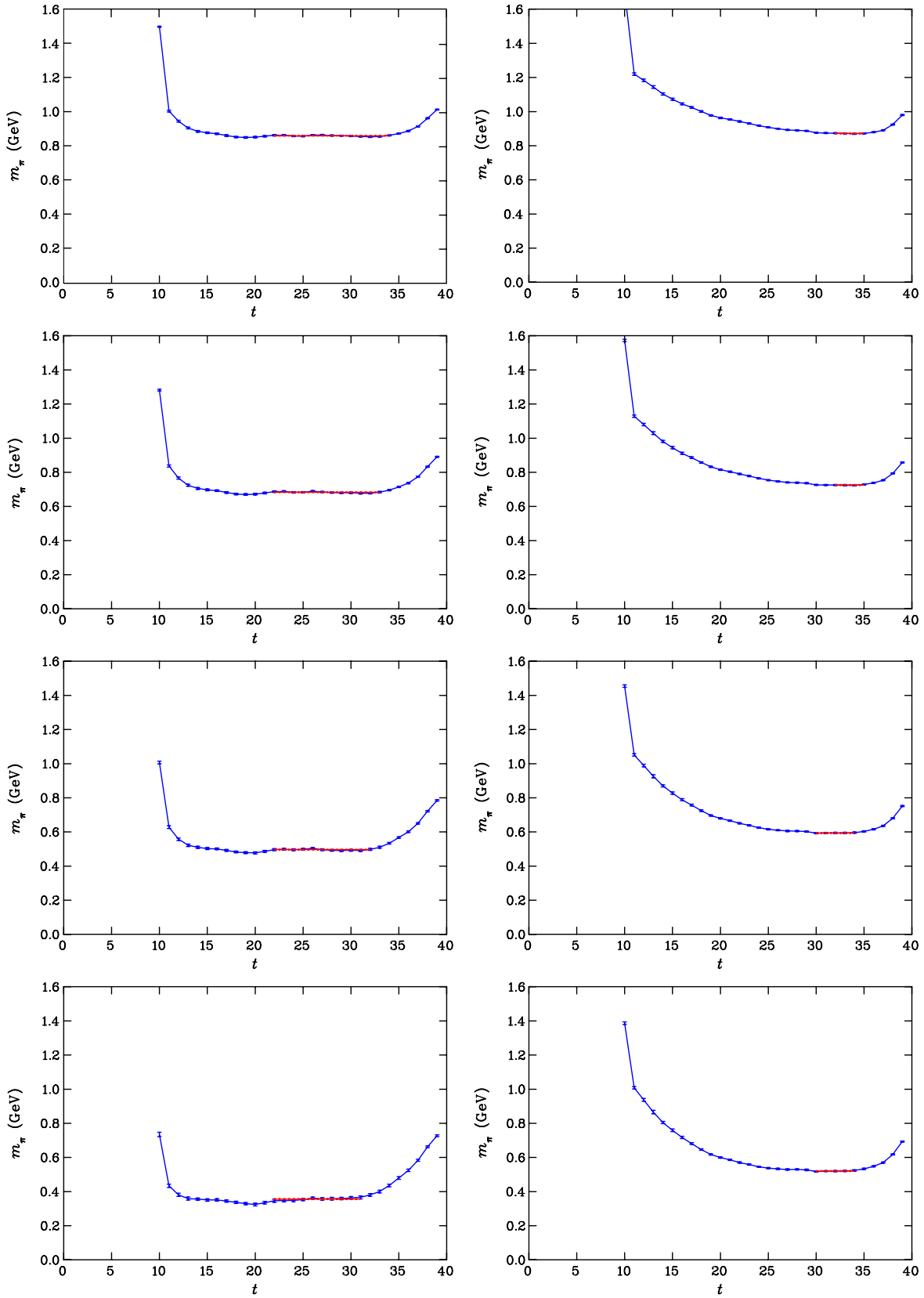
FIG. 1 (color online). Comparison of the pion effective mass evolution m(t) for the original configurations (left) and the vortex-free configurations (right) as the quark mass is decreased from the top downwards. The values of the hopping parameter \kappa are 0.1280 (top), 0.1293, 0.1304 and 0.1310 (bottom).
