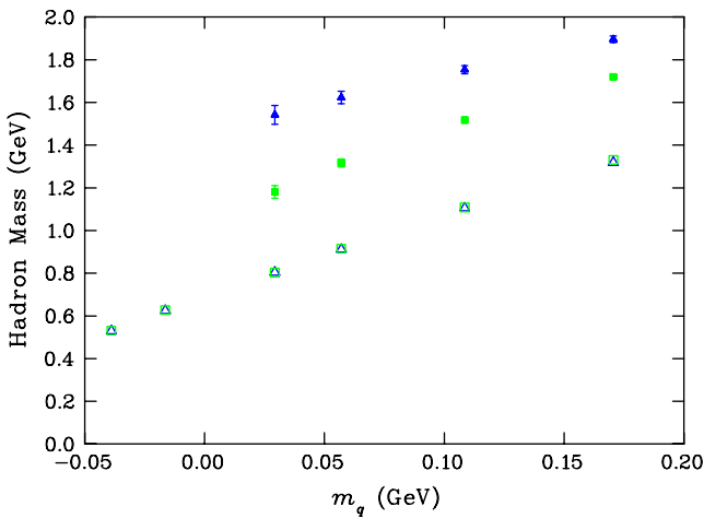
FIG. 6 (color online). Masses of the \Delta (triangles) and N (squares) from the original gauge-field configurations are compared with the masses from the vortex-free configurations. Full symbols illustrate results from the original configurations while the open symbols illustrate results from the vortex-free configurations.
