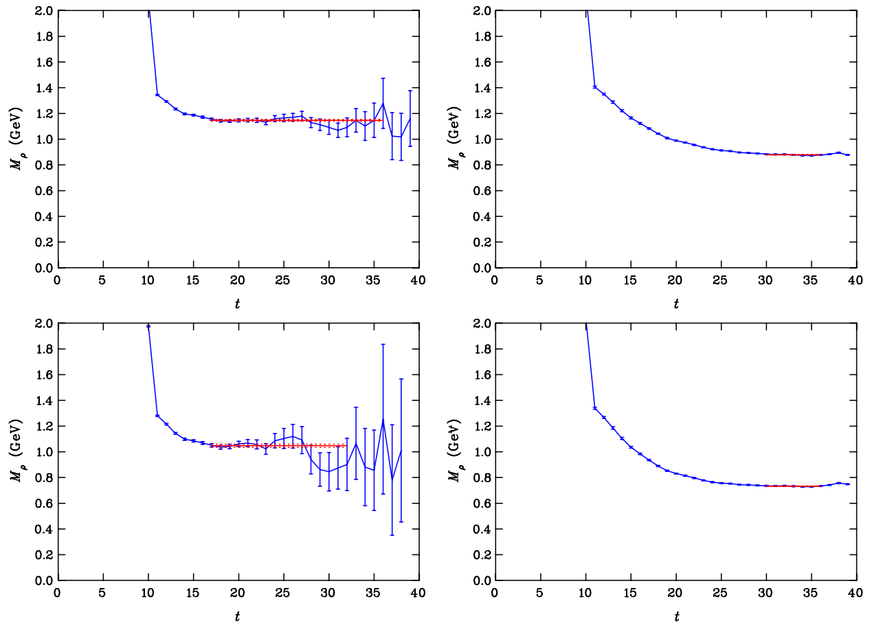
FIG. 2 (color online). Comparison of the \rho -meson effective mass evolution m(t) for the original configurations (left) and the vortex-free configurations (right) as the quark mass is decreased from the top downwards. The values of the hopping parameter \kappa are 0.1280 (top) and 0.1293 (bottom).
