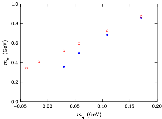
FIG. 4 (color online). Pion mass in GeV as a function of the bare quark mass determined with reference to the original configurations. Full symbols illustrate results from the original configurations while the open symbols illustrate results from the vortex-free configurations.
