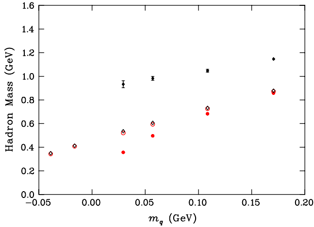
FIG. 5 (color online). Masses for the \pi (circles) and \rho (diamonds) mesons obtained from the original configurations (full symbols) and the vortex-free configurations (open symbols).
