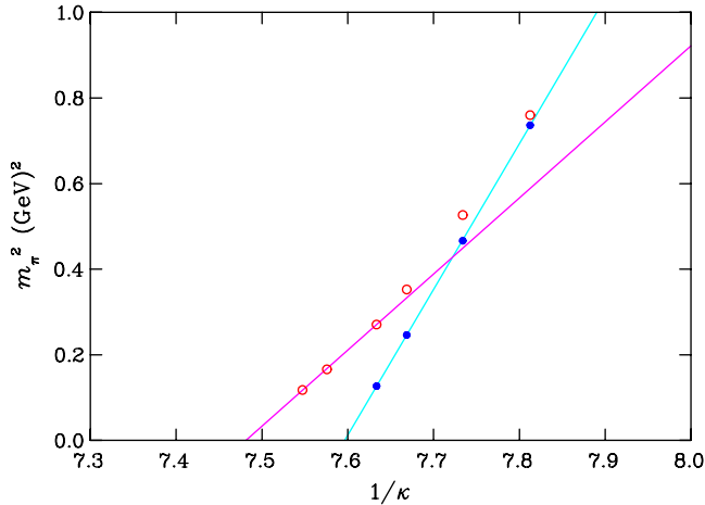
FIG. 3 (color online). Pion mass squared in terms of the inverse hopping parameter, \kappa^{-1} . The lines illustrate fits to the original configurations and the vortex-free configurations, the latter addressing only the lightest three quark masses considered where there is some promise that m_\pi^2 \propto \kappa^{-1} .
