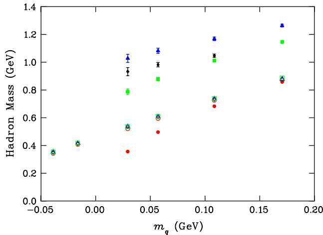
FIG. 8 (color online). The low-lying meson mass spectrum is compared with the low-lying baryon mass spectrum multiplied by 2/3 to account for the number of constituent quarks composing the system. Results from the original configurations (full symbols) and the vortex-free configurations (open symbols) are illustrated. The symbols are the same as in Fig. 7.
