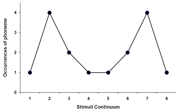
Figure 1: Distribution of stimuli used in phonetic training, defined along a continuum based on VOT. Tokens 2 and 7 occurred four times as often as tokens 1 and 8.
