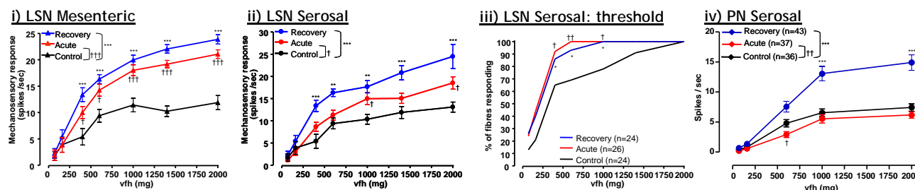
Figure 2. Specific classes of murine mechanosensitive colonic afferent become hypersensitive during and after inflammation. TNBS-induced colitis causes pronounced mechanical hypersensitivity in (A) high-threshold splanchnic (LSN): (A i) mesenteric afferents and (A ii) serosal afferents and (A iii) increases the percentage of afferents responding at a given stimulus intensity. These effects on mechanosensitivity become more apparent after resolution of inflammation (recovery; 30 days post-TNBS administration) when compared with acute conditions (7 days post-TNBS); (A iv) By contrast, pelvic (PN) high-threshold serosal afferents only become hypersensitivity following resolution from inflammation (recovery); (B) Low-threshold afferents display little or no change in mechanosensitivity after TNBS-induced colitis. Minor, but significant increases in mucosal responsiveness are observed in (B ii) mucosal and (B iii) muscular/mucosal afferents. By contrast, (B i) muscular and (B iii) muscular/mucosal afferent responses to stretch are unaffected by inflammation in the mouse. Modified from Hughes et al. , [37] with permission.
