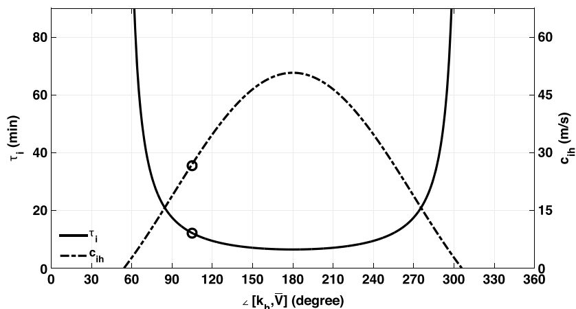
Figure 6. Intrinsic wave period (solid line) and intrinsic horizontal phase speed (dashed line) respective to the horizontal wind vector orientation at the altitude of the OH layer considering the background wind velocity \bar{V} = 32 m/s. The black circles correspond to the intrinsic parameters for the wave segment highlighted in Figure 3.
