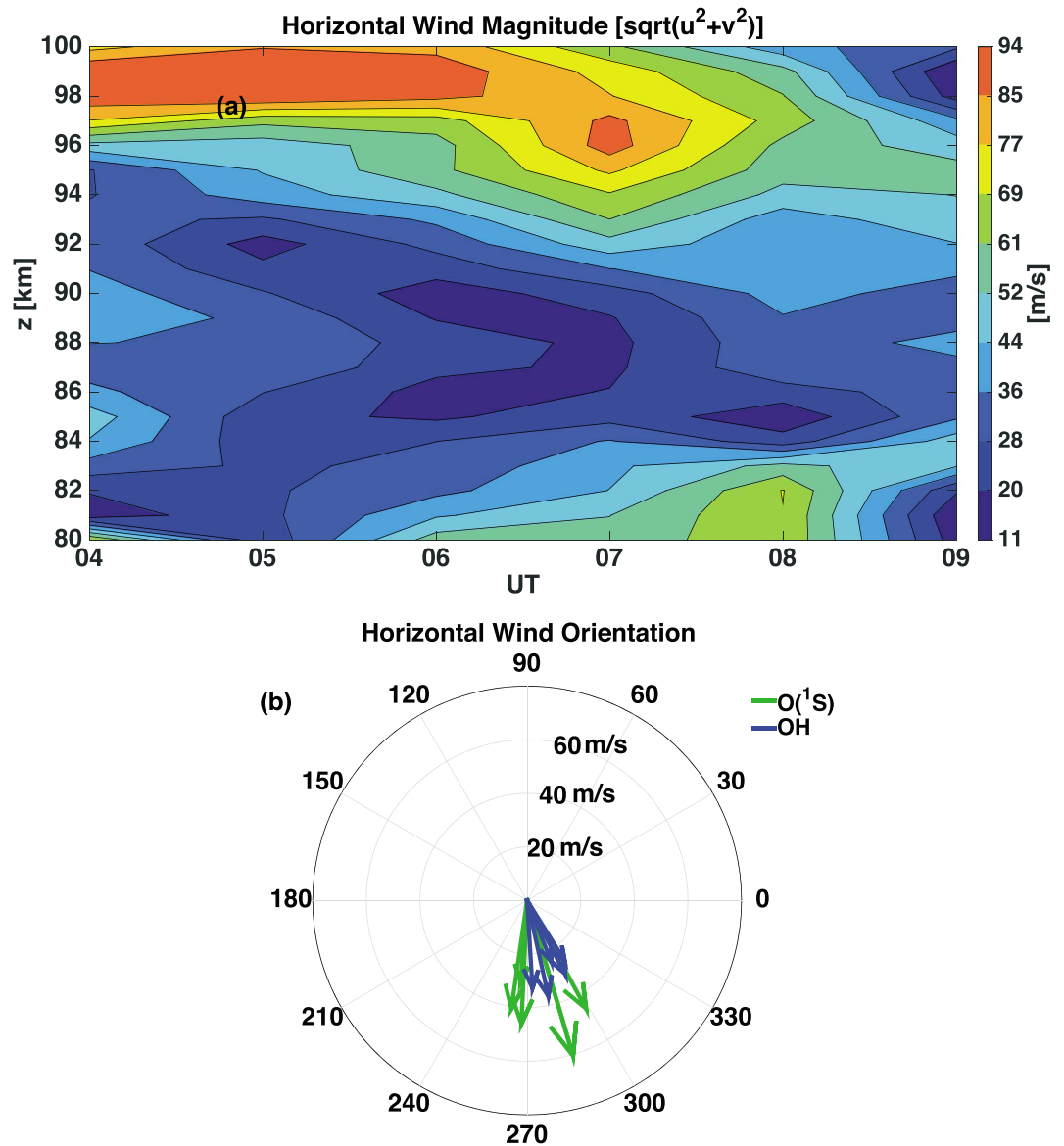
Figure 5. (a) Cross section of the horizontal wind magnitude measured by the ALO meteor radar system and (b) horizontal wind orientation at the peak of the OH and O(^1S) layers. The horizontal wind at the OH and O(^1S) was obtained assuming the layer centroid at 87.8 and 96 km, respectively.
