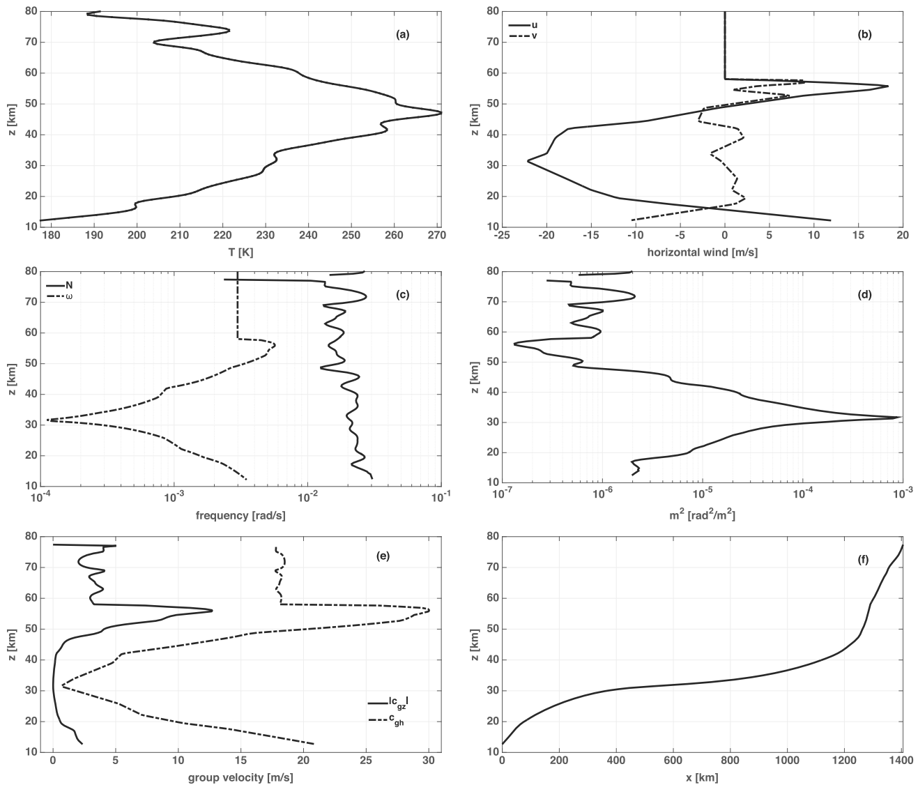
Figure 12. Forward ray tracing of the primary wave originated ~1400 km from ALO over Bolivia region (20.4°S, 56.2°W). (a) SABER satellite temperature (event number 93, orbit number 55736, 03:01:53 UT); (b) instantaneous 3-hourly 1.25° zonal and meridional winds (MERRA model MAI3CPASM v5.2.0); (c) altitude variation of the Brunt-Väisälä frequency and the primary wave frequency due to nonisothermic and nonstatic atmospheric structure (notice the critical level between 75 to 80 km altitude); (d) primary wave squared vertical wave number and (e) the vertical and horizontal group velocity. (f) Primary wave x-z trajectory from its source in the lower atmosphere to the critical level observed at 80 km altitude. Notice that the MERRA model provides winds up to 60 km only; we have assumed u(z) = v(z) = 0 m/s above that level.
