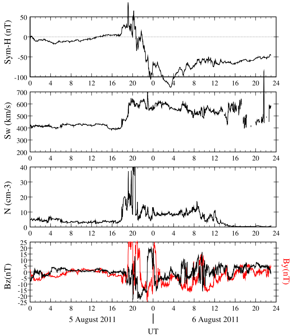
Figure 4. Same as Figure 1 but corresponding to 5–6 August 2011.
