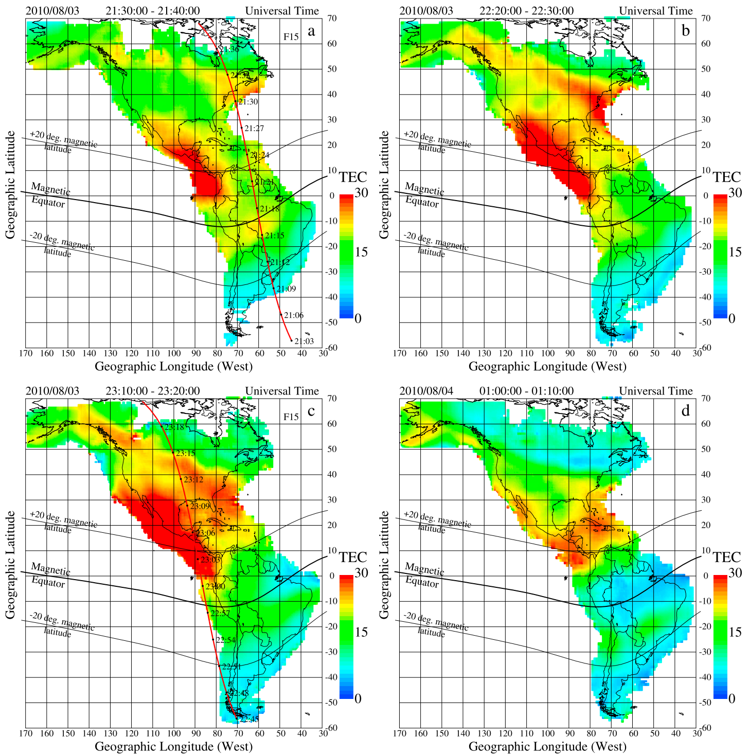
Figure 2. Total electron content measured by the LISN and several networks of GPS receivers that operate in North, Central and South America, and the Caribbean region. The four frames correspond to the following times: (a) 21:30–21:40 UT, (b) 22:20–22:30 UT, (c) 23:10–23:20 UT, and (d) 01:00–01:10 UT. Figures 2a and 2c show the trajectory of two consecutive passes of DMSP-F15.
