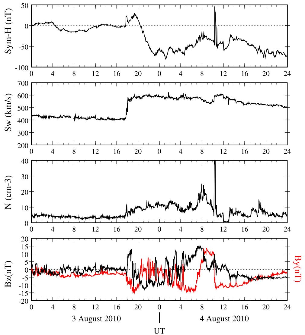
Figure 1. SYM-H index and interplanetary data corresponding to the storm event of 3–4 August 2010. The interplanetary data were measured by the ACE satellite. From top to bottom, the four frames show the 1 min SYM-H index (nT), the solar wind velocity (km/s), the solar wind proton density ( \text{cm}^{-3} ), and the IMF B_z and B_y components (nT) displayed in black and red.
