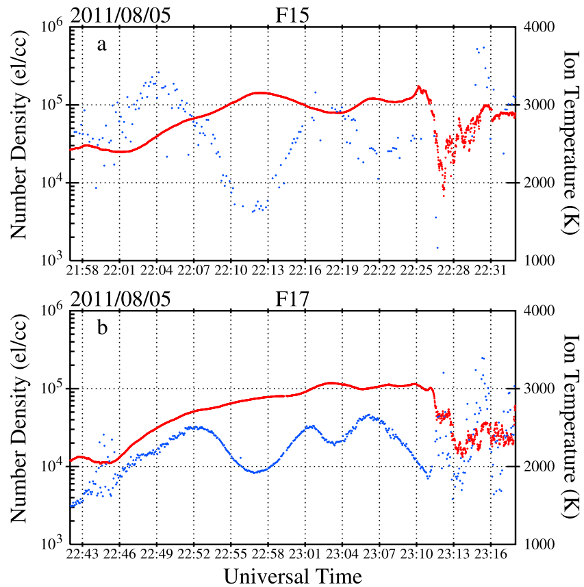
Figure 6. Same as Figure 3 but corresponding to 5–6 August 2011.
