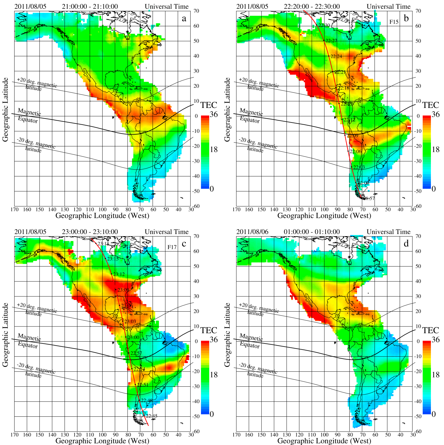
Figure 5. Same as Figure 2 but corresponding to 5–6 August 2011. GPS TEC maps for (a) 21:00–21:10, (b) 22:20–22:30, (c) 23:00–23:10, and (d) 01:00–01:10 UT. Figures 5b and 5c show passes of the DMSP-F15 and F17, respectively.
