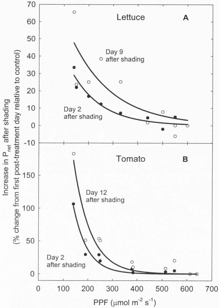
Figure 4-2. Recovery of net photosynthesis ( P_{\text{net}} ) recovery for lettuce and tomato. These data are from all ten chambers, and are expressed as a percent of initial P_{\text{net}} after shading treatments were imposed.
