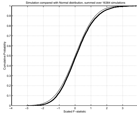
Figure 2. Partial convergence of the F-statistic to a normal distribution. The heavy line is based on data points from a large simulation based on the null hypothesis. The fine line is calculated using the scaling law, stated in Abramowitz and Stegun. The convergence is good, even for small sample sizes of the type found in the Iliad .
