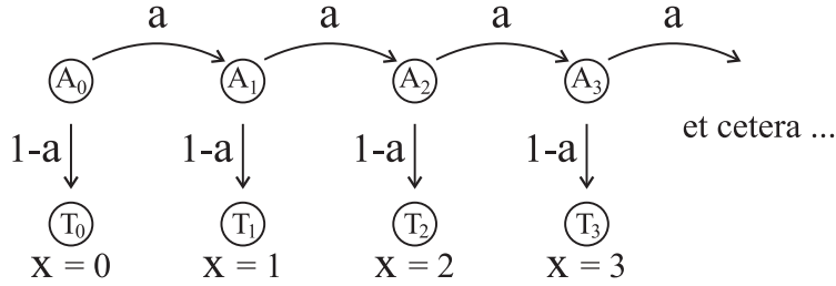
Figure 1. The discrete Poisson process, as a Markov chain: The initial state is A_0 , which means ‘active with x = 0 .’ This corresponds to the state where no words have yet been examined. In general, the state A_k refers to an active state with x = k . Physically, this corresponds to the case where we have examined k words and none of them were the proposed keyword. All states marked ‘A’ are active, meaning that we are still actively searching for the next instance of the proposed keyword. The state T_k refers to the terminal state with x = k . Physically, this corresponds to the case where we have examined k + 1 words and the first k words were not the proposed keyword and the last word was the desired keyword. All states labelled ‘T’ are terminal, meaning that the Markov chain has now terminated. The labels on the arrows refer to the conditional probabilities of transition from one state to another. The conditional probability that a word is not used, in any active state, is a and the conditional probability that the word is used is 1 - a . All events are independent, so if the probability of arriving at the initial state, A_0 , is 1 then the probability of arriving at state T_k , with x = k , is P(x) = (1 - a) \cdot a^x . After the Markov chain has terminated, it immediately restarts again at state A_0 , with probability of one, and the whole procedure is repeated until the end of the text is reached. This Markov chain can also be used to generate pseudo-random numbers in order to simulate the null hypothesis.
