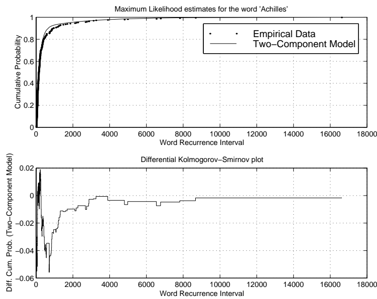
Figure 6. A Kolmogorov-Smirnov plot of empirical data for the word ‘Achilles’, from the translation of the Iliad by Lang. 4 The bottom half shows a plot of the difference between the distribution implied by a two-component mixture distribution and the empirical distribution of the data. The Kolmogorov-Smirnov statistic is now 0.0558, which is quite probable, given the new model. The empirical data is identical with that used in Figure 4, only the model has changed.
