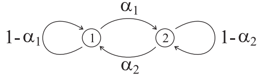
Figure 7. A two-state Markov process: This is one possible mechanism for producing the mixture of two discrete Poisson processes. When the process is in ‘state 1’ the first Poisson process is active and has the parameter value a = a_1 and when the process is in ‘state 2’ the second Poisson process is active and has the parameter value a = a_2 . This gives rise to frequent changes in the value of the parameter, a , which generates a random variable with the long-term time-average density function described in Equation 9.
