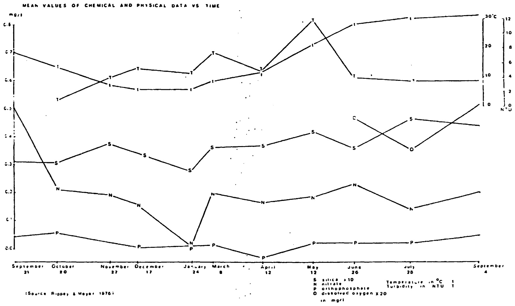
Figure 2. Temporal distribution of mean values for selected physico-chemical parameters.
