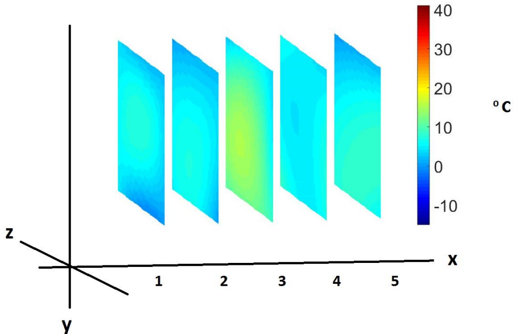
Figure 14. A thermal map of average temperatures for each location throughout the trailer (see figure 1) when plastic wrap was used* within the second half of the trip duration#
