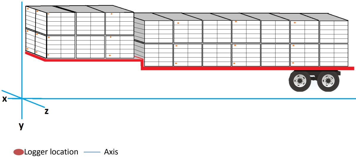
Figure 1. Schematic of an industry standard drop deck poultry trailer loaded with 20, 10 door modules
