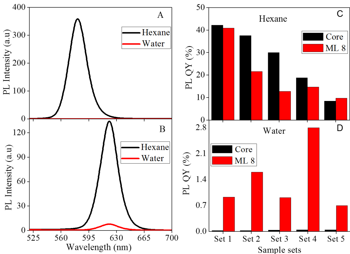
Figure 3.6. (A and B) Photoluminescence spectra of the sample set 3 for both the core and ML 8, respectively, before (hexane) and after ligand exchange (water). Photoluminescence quantum yields histograms before (C) and after ligand exchange using 3-mercaptopropionic acid (MPA) (D) for the sample sets 1- 5. There is a complete quenching of the core samples after ligand exchange compared to their ML 8 counterparts.
