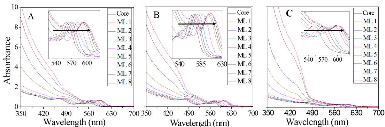
Figure 3.1. Absorbance spectra as a function of shell thickness (number of monolayers) for samples sets 1(A), 3(B) and 5(C). For each of these samples there is a steady redshift shown by the arrows depicting shell growth.
