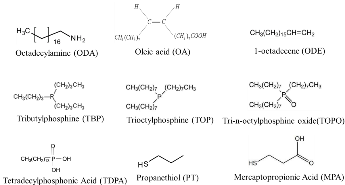
Figure 1.5. Common ligands used as coordinating and non-coordinating ligands during synthesis and ligand exchange of quantum dots.
