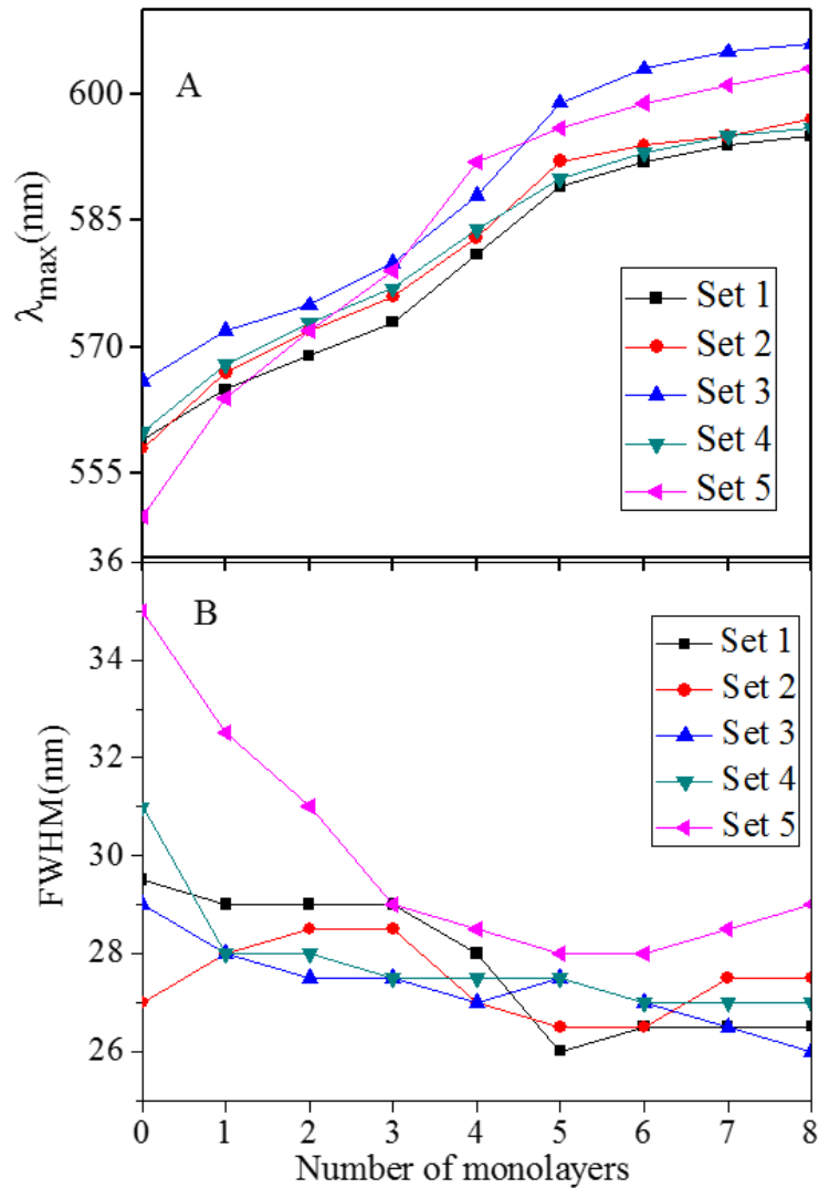
Figure 3.2. (A) Absorbance \lambda_{\max} as a function of number of monolayers for the sample sets 1-5 illustrating the extent of redshift as the shell grows thicker. (B) Full width at half maximum (FWHM) as a function of the number of monolayers for the sample sets 1 – 5 showing a constant distribution in size before and after shelling.
