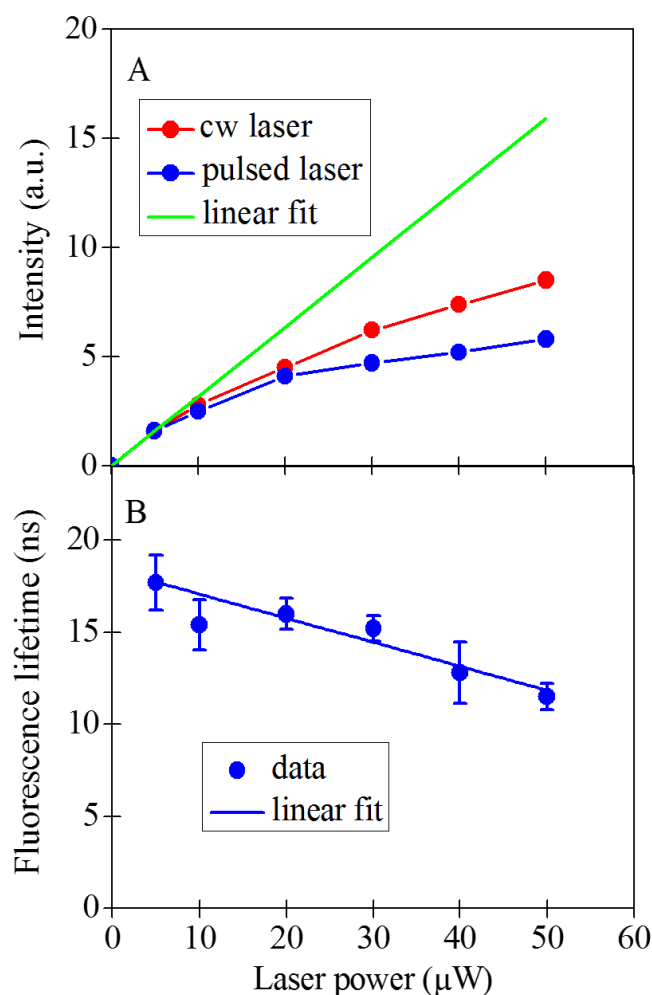
Figure 4.1. (A) The comparisons of fluorescence intensities of single QDs in PMMA matrix from cw laser or pulsed laser excitation. (B) The fluorescence lifetimes of single QDs decrease slightly over the laser power range of 5-50 \mu\text{W} .
