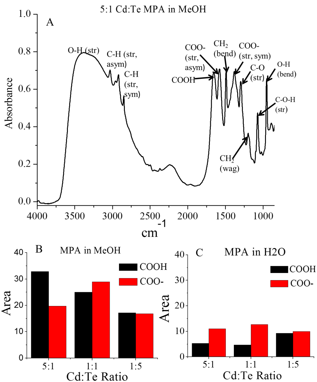
Figure 2.5. (A) FT-IR absorption spectrum of MPA exchanged CdTe in methanol, synthesized with a Cd:Te ratio of 5:1. (B and C) COOH (black) and COO - (red) for MPA-exchanged CdTe in methanol and water, respectively, as a function of Cd:Te ratio.
