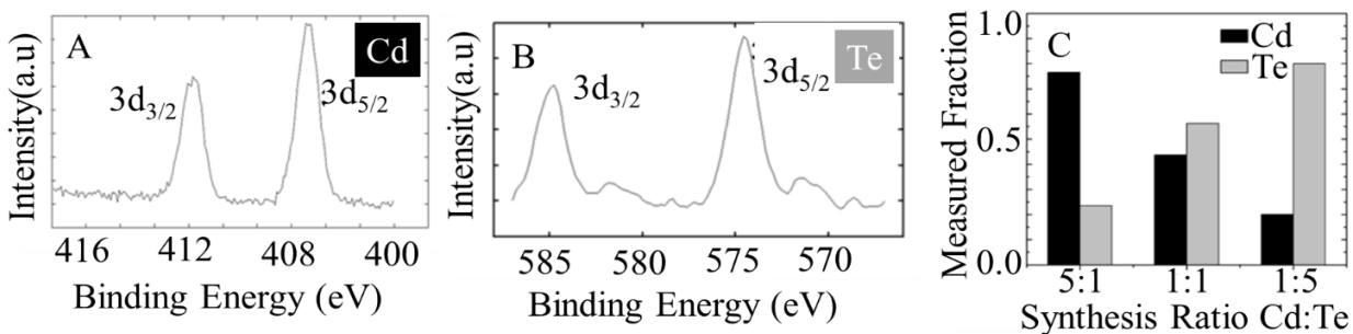
Figure 2.2. (A) XPS spectra of Cd peaks from 5:1 Cd:Te QDs. (B) XPS spectra of Te peaks from 1:5 Cd:Te QDs. (C) Integrated peak areas of Cd and Te, normalized to a total fraction of 1, for 5:1, 1:1, and 1:5 Cd:Te.
