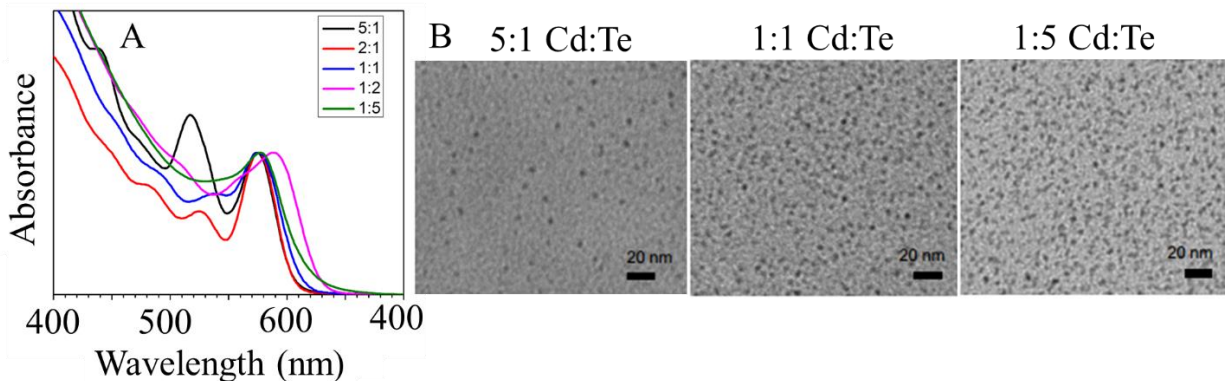
Figure 2.1. (A) Absorption spectra of CdTe QDs with varying Cd:Te ratios. (B) TEM images of Cd-rich, CdTe neutral and Te-rich CdTe QDs
