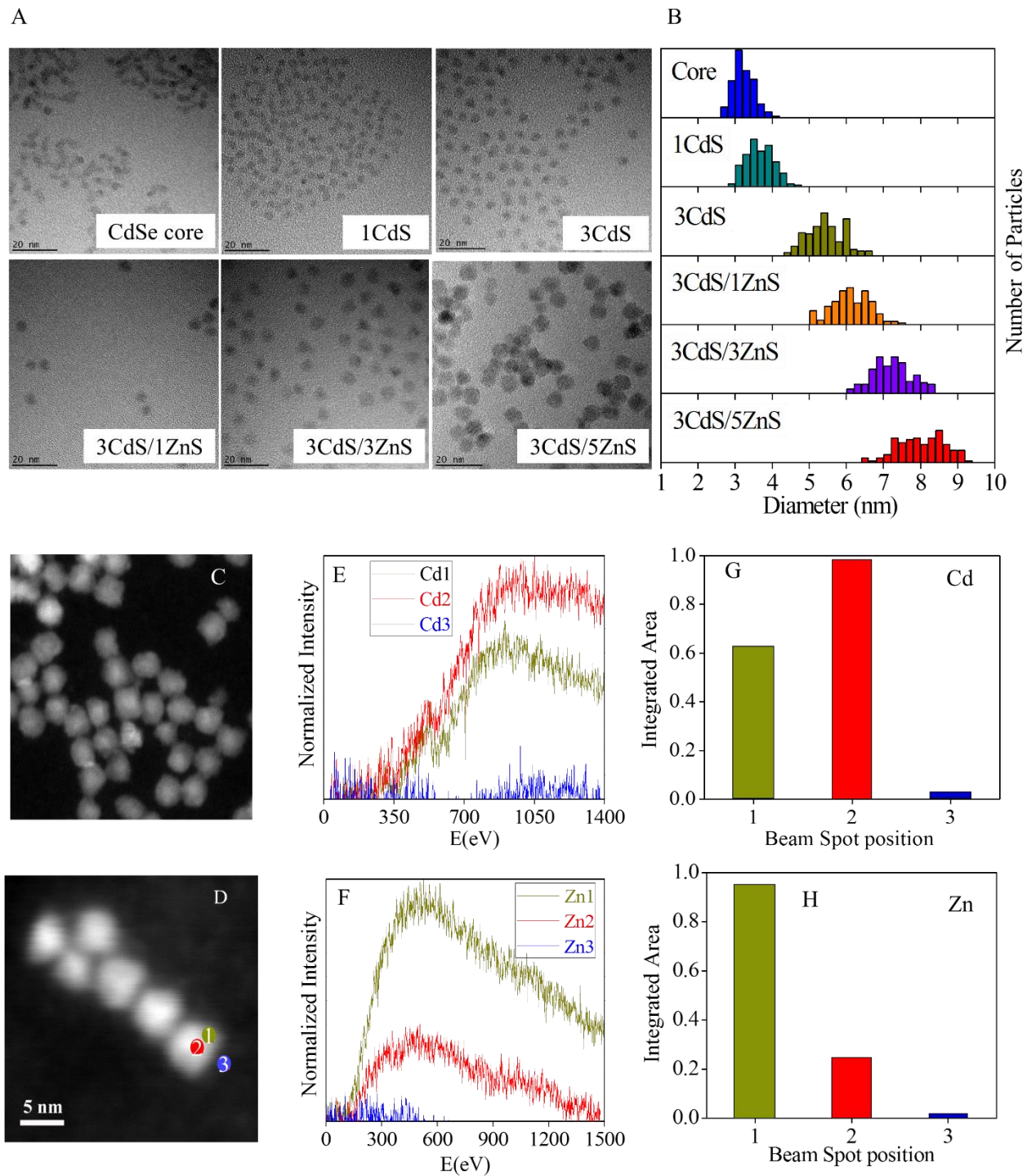
Figure 4.4. (A) TEM images of the selected samples together with their respective size distribution histogram (B), (C and D) Annular dark field (ADF)-STEM images of the CdSe/3CdS/5ZnS core/shell/shell sample. (E and F) are the electron energy loss spectra (EELS) of Cd and Zn signals, respectively, collected at positions indicated in figure 4.4D. (G and H) are the integrated area histograms calculated from the spectra in figures E and F, respectively.
