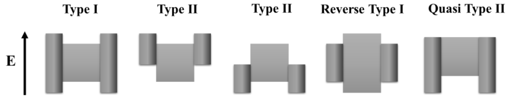
Figure 1.2. Schematic of band gap energy overlap in different types of core/shell quantum dots. The inner rectangular blocks represent the cores while the outer ones represent the shell band-gap energies, respectively.
