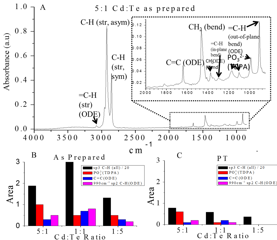
Figure 2.4. (A) FT-IR absorption spectrum of as-prepared CdTe synthesized with a Cd:Te ratio of 5:1. (B and C) Integrated peak areas of the sp 3 C–H peak (black), PO 3 2- peak from TDPA (red), and two peaks that are representative of ODE ligands, C=C (blue) and the sp 2 C–H (magenta) for as-prepared and PT-exchanged CdTe, respectively, as a function of Cd:Te ratio.
