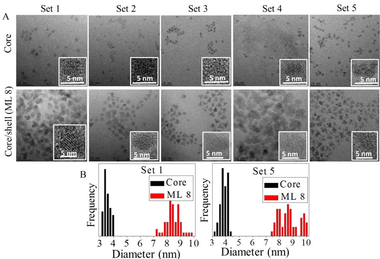
Figure 3.4. (A) TEM images of CdSe core and corresponding CdSe/8ML CdS core/shell quantum dots for all the sample sets 1- 5. Inset is the respective HRTEM image of each sample revealing high crystallinity of the samples. (B) Size distribution histograms of sets 1 and 5 for both core and ML 8 core/shells, showing the average diameter and size dispersity of the quantum dots.
