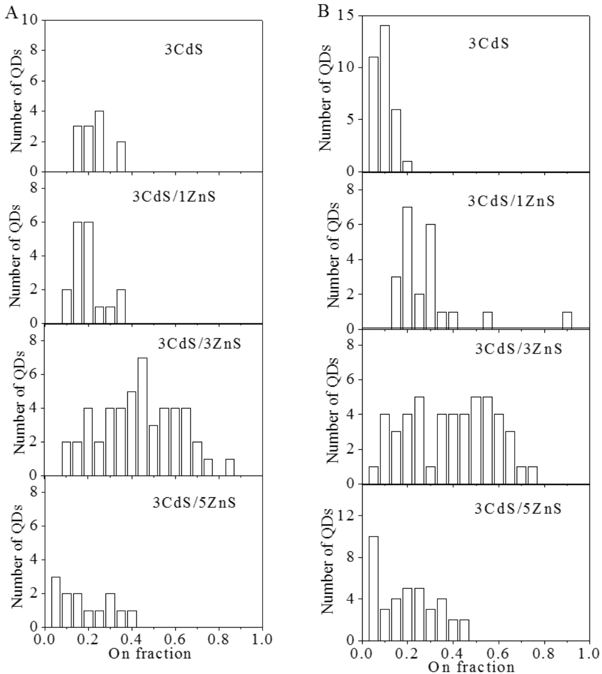
Figure 4.8. On-fraction distributions for CdSe/CdS/ZnS QDs having 3 monolayers of CdS and different thickness of ZnS shells. (A) under cw laser excitation and (B) under pulsed laser excitation.
