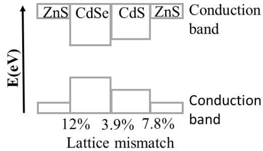
Figure 1.3. Lattice mismatch and band gap overlap of semiconductor quantum dots as used in chapter 4.
