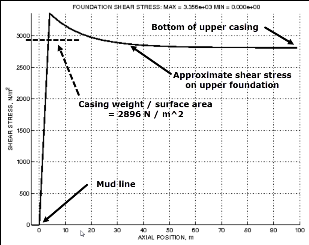
Fig. 5 Approximate shear stresses in upper sediments from upper casing weight
