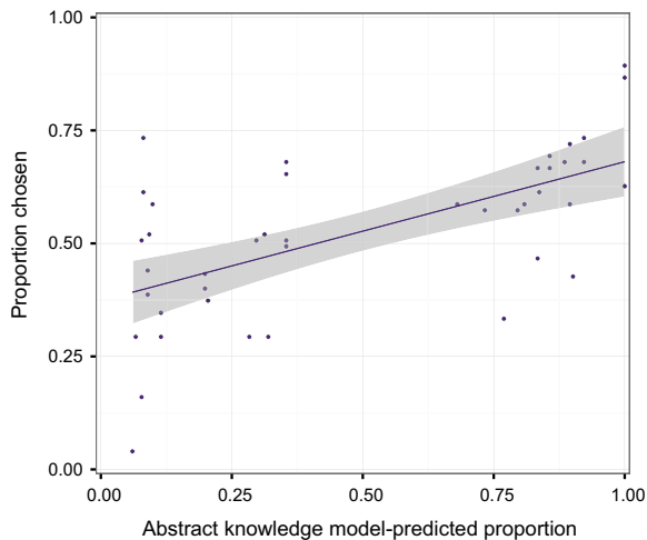
Fig. 3. Results of Experiment 1 (novel items): Ordering preferences for novel binomials by model-predicted abstract knowledge. Each point represents an item. x values are the abstract knowledge model's prediction for how often the item will appear in alphabetical order. y values are how often the item was preferred in that order. Line shows best linear fit on the by-items aggregated data. Abstract knowledge is a significant predictor of preferences for novel expressions.
