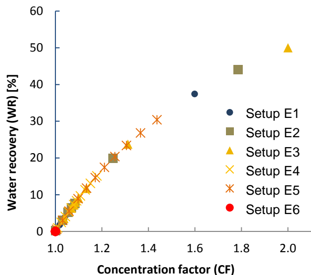
Fig. 10. Water recovery versus concentration factor.
