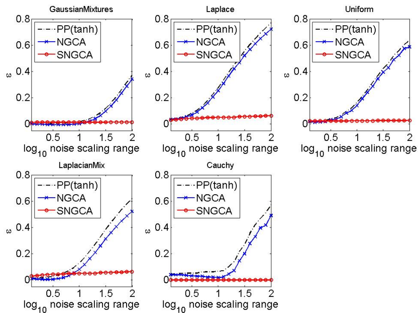
Fig. 3 estimation error with respect to the standard deviation of Gaussian components following a geometrical progression on [10^{-\tau}, 10^{\tau}] where \tau is the parameter on the abscissa
