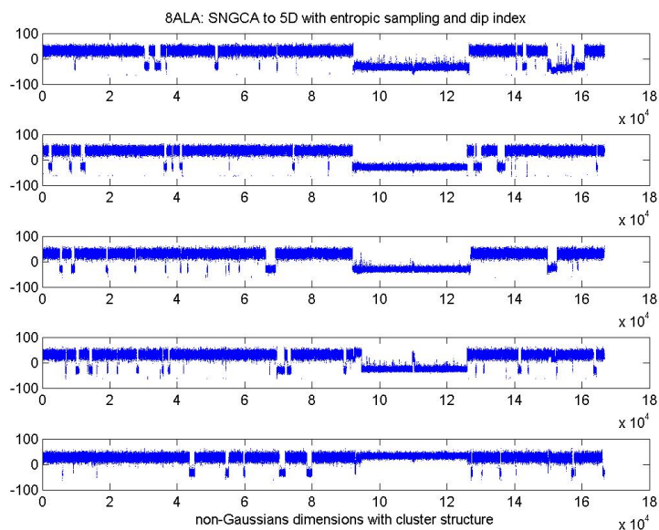
Fig. 5 low dimensional multimodal component of 8-alanine
