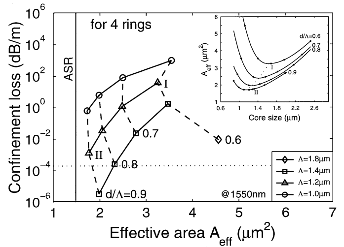
Fig. 3. Confinement loss versus effective mode area for a range of \Lambda and d/\Lambda with four rings. The solid vertical line represents the minimum mode area for the limit of a silica ASR. Inset: mode area for a range of HFs as a function of the core size ( 2\Lambda - d ).
