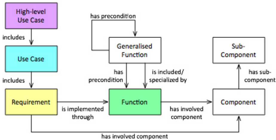
Fig. 1 Entities and relationships involved in the analysis of requirements
