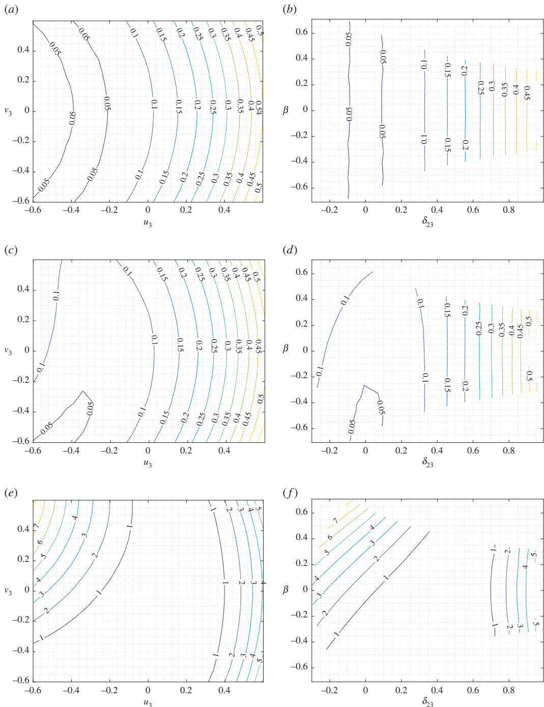
Figure 6. King post truss: level sets for the strain energy W for \delta_{12} = -0.3 varying a in the plane u_3 – v_3 ( a, c, e ) and in the plane \delta_{23} – \beta ( b, d, f ). ( a, b ) a = 0.01 , ( c, d ) a = 1 and ( e, f ) a = 100 .
