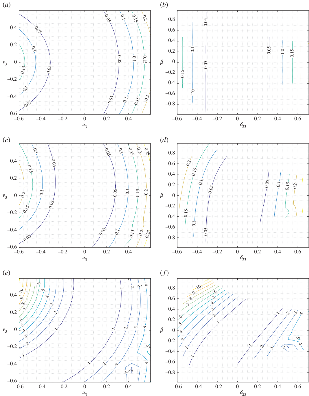
Figure 7. King post truss: level sets for the strain energy W for \delta_{12} = 0 varying a in the plane u_3 - v_3 ( a, c, e ) and in the plane \delta_{23} - \beta ( b, d, f ). ( a, b ) a = 0.01 , ( c, d ) a = 1 and ( e, f ) a = 100 .
