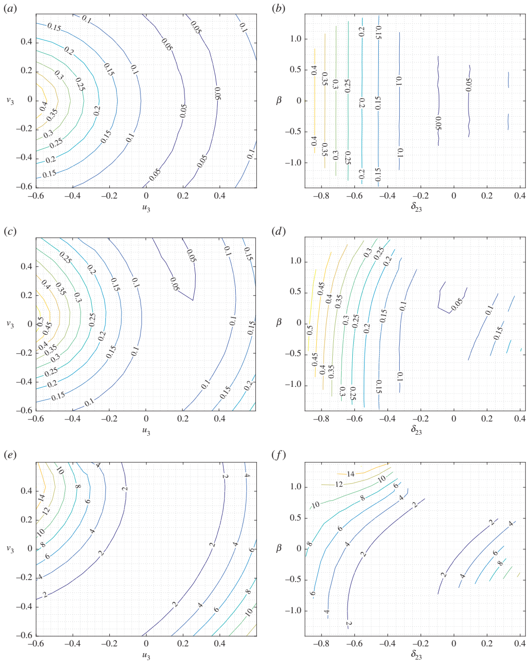
Figure 8. King post truss: level sets for the strain energy W for \delta_{12} = 0.3 varying a in the plane u_3 - v_3 ( a, c, e ) and in the plane \delta_{23} - \beta ( b, d, f ). ( a, b ) a = 0.01 , ( c, d ) a = 1 and ( e, f ) a = 100 .
