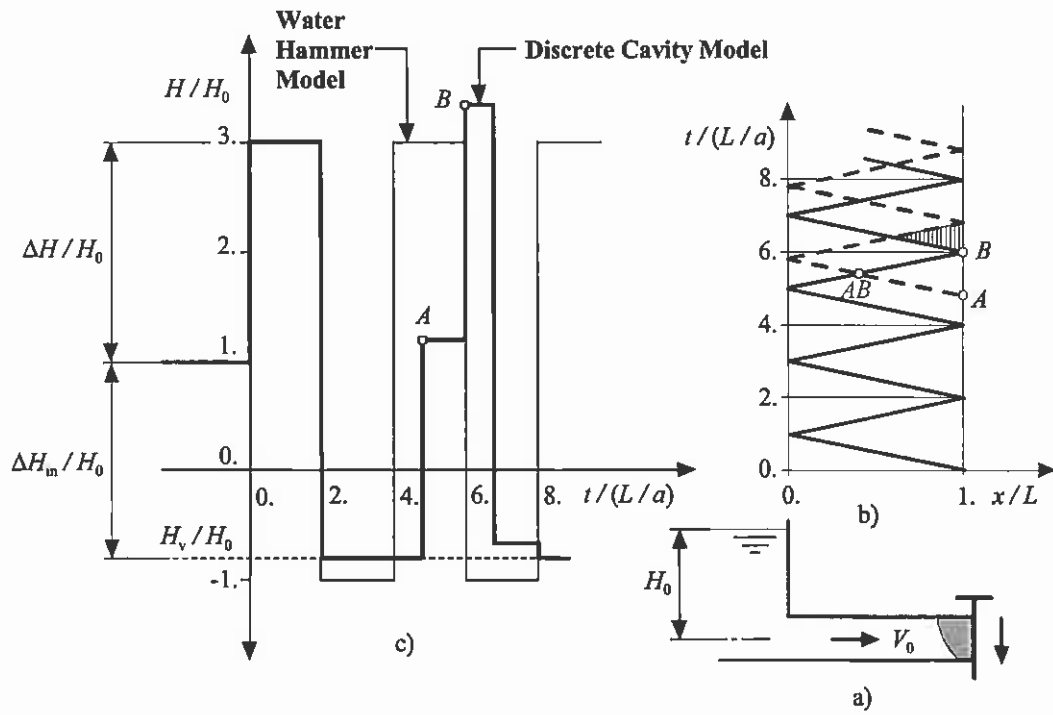
Fig. 3 Formation of a short-duration pressure peak. (a) Reservoir-pipe-valve system. (b) Wave paths in distance-time plane. (c) Piezometric-head history at valve.
