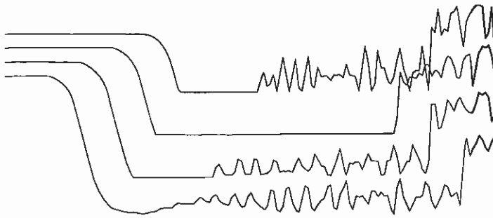
Fig. 10 Numerical oscillations in DVCM results (adapted from De Vries, 1972, Fig. 42). Pressure-head histories at different positions after pump shutdown.
