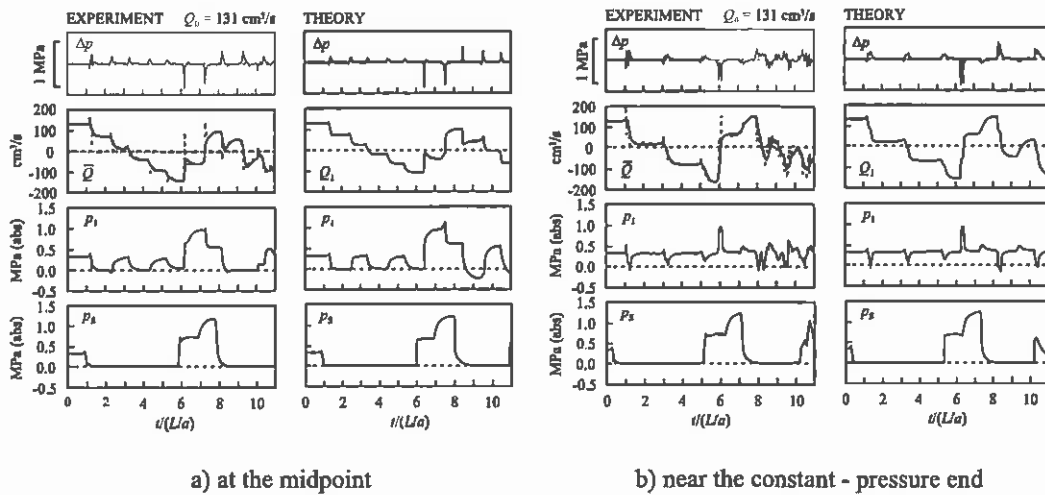
Fig. 17 Measured (first and third column) and calculated (second and fourth column) results in column-separation experiment. The second row depicts flow rates (adapted from Washio et al., 1996, Fig. 8).
