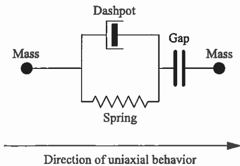
Fig. 15 DVCM in FEM context (adapted from Schwirian, 1984, Fig. 4). Dynamic element with gap, which allows the formation of a cavity.
