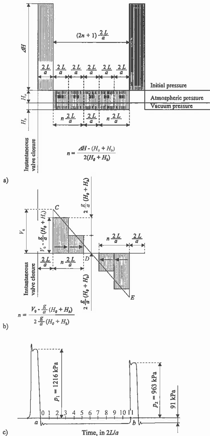
Fig. 7 Theoretical and experimental analysis of column separation in a reservoir-pipe-valve system.
