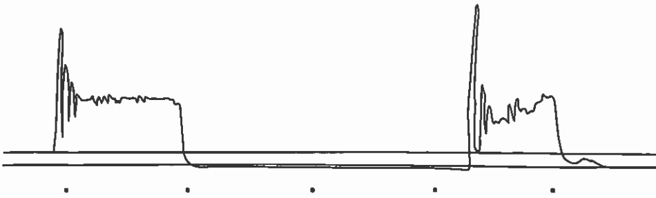
Fig. 1 Pressure record exhibiting column separation. Horizontal axis: time (each dot indicates half a second). Vertical axis: pressure (Joukowsky pressure of 15.3 bar). The upper horizontal line is the static pressure and the lower horizontal line is the atmospheric pressure. (adapted from Joukowsky, 1900, Fig. 17; also shown by Simin, 1904, Fig. 13, and by Moshnin and Timofeeva, 1965, Fig. 1)
