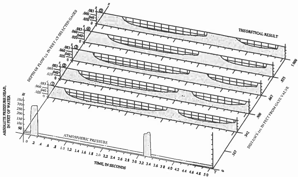
Fig. 13 Simulated transient pressures at gate valve and concurrent, free-surface profiles of vapor cavity (adapted from Baltzer, 1967b, Fig. 4).
