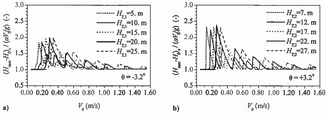
Fig. 5 Computed maximum head at valve as function of initial velocity for varying reservoir-head (adapted from Bergant and Simpson, 1999a): (a) downward sloping pipe, (b) upward sloping pipe.
