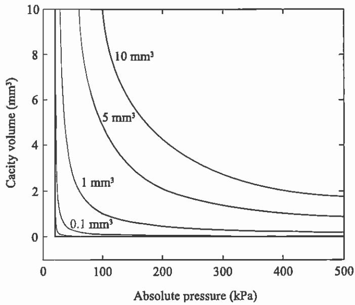
Fig. 11 p^* - V curves for DVCM (thick solid line, V_0 = 0 \text{ mm}^3 ) and DGCM (thin solid lines, V_0 = 0.01 \text{ mm}^3 , V_0 = 0.1 \text{ mm}^3 , V_0 = 1 \text{ mm}^3 , V_0 = 5 \text{ mm}^3 , V_0 = 10 \text{ mm}^3 ) with p_0^* = 1 \text{ bar} and p_v^* = 0.2 \text{ bar} . The value of p_v^* (water at 60 \text{ }^\circ\text{C} ) is chosen large to show its influence.
