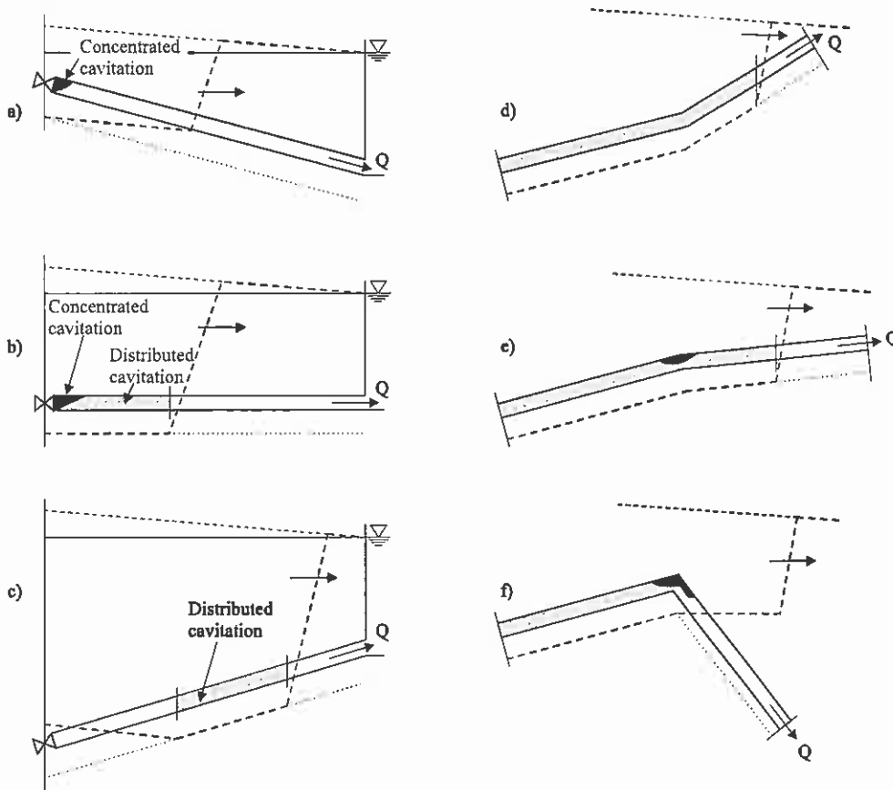
Fig. 2 Dotted lines: vapor head; thin dashed lines: steady-state head; dashed lines: unsteady head.
