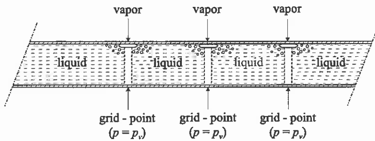
Fig. 9 Definition sketch for discrete vapor cavity model (adapted from Tijsseling, 1993, Fig. 4.9)
