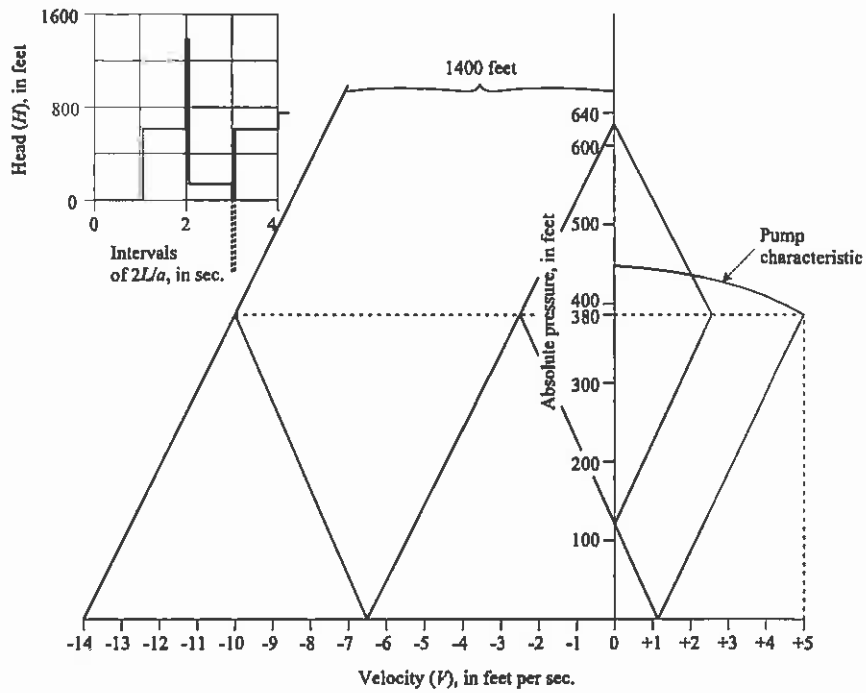
Fig. 8 Graphical method (adapted from Angus, 1937, Fig. 20).
