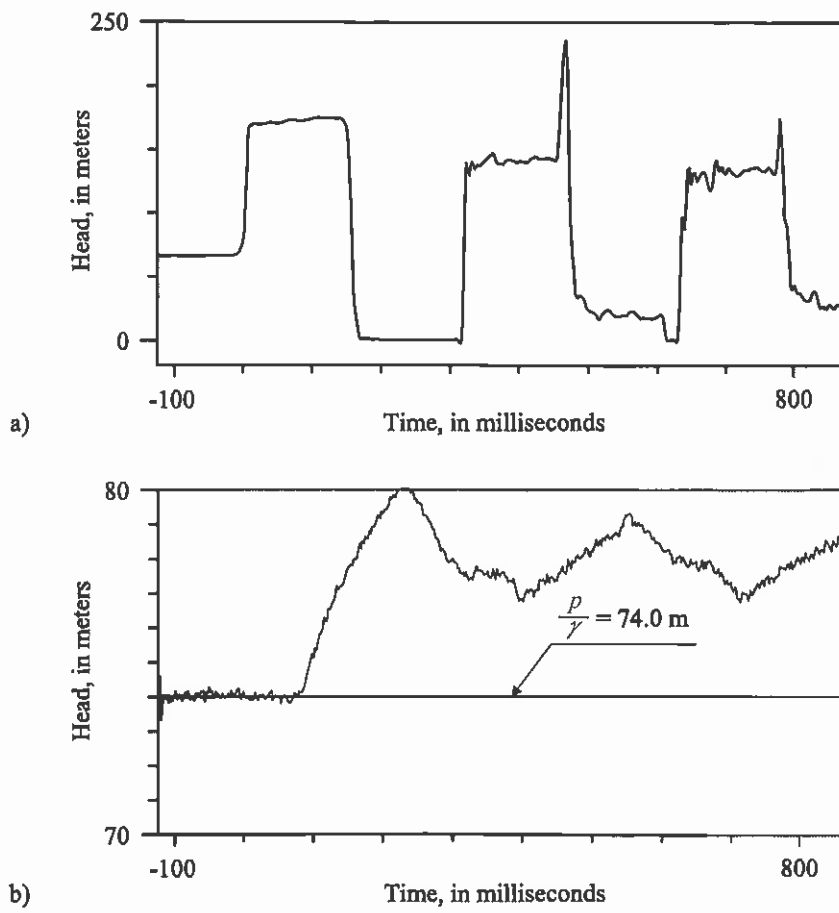
Fig. 4 Experimental result showing short-duration pressure peaks (adapted from Martin, 1983, 1989). Absolute hydraulic grade line (HGL) variation with time, (a) at valve, and (b) in reservoir.
