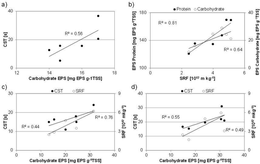
Fig. 2. Correlation during Phase V: CST vs specific bound carbohydrates EPS in aerobic reactor (a); specific bound proteins and carbohydrates EPS vs SRF in anoxic reactor(b); CST and SRF vs specific bound carbohydrates EPS in aerobic reactor (c); CST and SRF vs specific bound carbohydrates EPS in MBR reactor (d)
