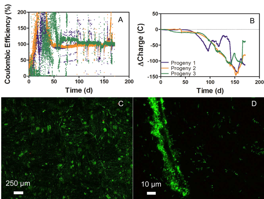
Figure 2. (A) Coulombic efficiency of each cycle over the duration of the experiment. A cycle is defined as each 20 min period consisting of 10 min poised at a cathodic potential ( -0.4 V) followed by 10 min poised at an anodic potential ( 0.0 V). Here, each point represents the ratio of the charge produced as an anode to the charge consumed as a cathode during each 20 min period. It should be noted that significant current was not produced until approximately day 50. Accordingly, CE data obtained prior to day 50 are difficult to interpret. After day 50, the bulk of the noise occurs when the medium was exchanged in the reactors. (B) Net change in charge over the duration of the experiment. Charge consumed as a cathode was subtracted from the charge produced as an anode resulting in a net imbalance of charge skewed toward the cathodic reaction (depicted as negative here). We should note that the overall net change in charge is small compared to the total charge passed through the system over the duration of the experiment ( 6250 \pm 750 C as an anode and 6300 \pm 800 C as a cathode). (C and D) Confocal laser scanning microscope images of the biofilm on the electrode surface treated with Live/Dead stain taken with 10\times and 60\times objectives, respectively. The green fluorescence indicates an intact cell membrane.
