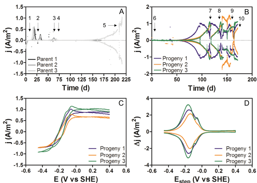
Figure 1. (A) Development of the nonphotosynthetic bifunctional electrode in parent reactors. Numbers on the graph correspond to (1) inoculation and addition of 5 mM acetate, (2) addition of 1 mM acetate, (3) the first indication of bidirectional current, (4) parents 1 and 2 killed, and (5) maximum bifunctional current density production by parent 3. (B) Development of the bifunctional electrode in the progeny reactors. Numbers on the graph correspond to (6) inoculation from parent 3, (7) medium replacement, (8) medium replacement and electrode sampling from progeny 3 for confocal microscopy, (9) electrode sampling from progeny 1 and 2 for confocal microscopy, and (10) CV and SWV depicted in panels C and D. (C) Voltammograms of triplicate reactors taken at the end of the experiment (point 10 in panel B) exhibiting bifunctionality on the anodic and cathodic limits of the scan. (D) Square wave voltammograms exhibiting two reversible redox peaks at -0.15 and -0.05 V, although the peak at -0.15 V is clearly dominant.
