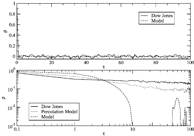
FIG. 12. Autocorrelation functions for the fluctuations r (top) and the volatility \nu (bottom). The parameters used to produce the analyzed set are N=10^4 nodes, \theta=0.9 for the clustering probability, m=m_0=5 for the links of each new node, a=1.8 and \kappa=a for the group and global opinion response, respectively.
