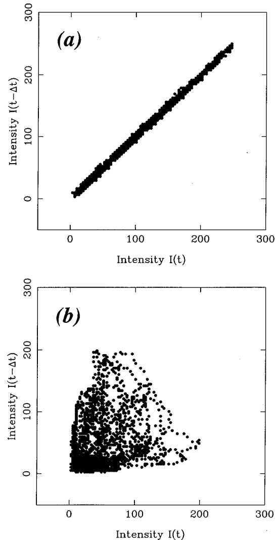
FIG. 3. Relationship plot of the laser dynamics shown in Fig. 2 under repeated drivings. \Delta t is the repetition period of driving signal, which is 150 \mu\text{s} in our experiment. (a) Relationship plot of the driving signal; (b) relationship plot of the laser dynamics.
