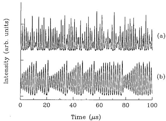
FIG. 2. Chaotic dynamics of the laser without generalized synchronization of chaos to the driving signal. The average pump-laser intensity is 0.8 \text{ W/cm}^2 and the gas pressure is 19 \mu\text{bar} . Peak-peak pump intensity modulation strength is 28% of the mean pump intensity. (a) Chaotic laser intensity evolution; (b) evolution of the chaotic driving signal measured.
