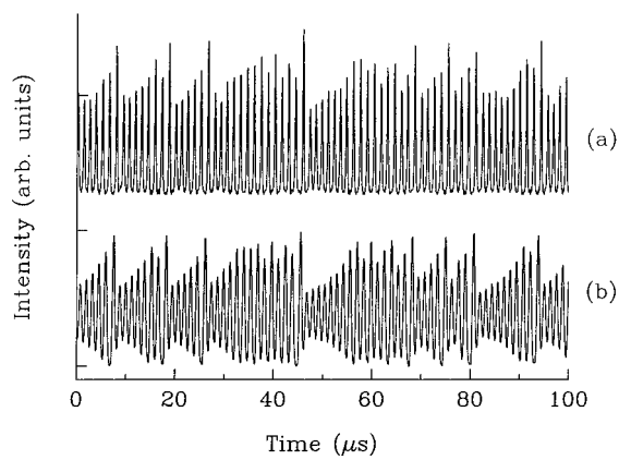
FIG. 6. Chaotic dynamics of the laser under the generalized synchronization of chaos to the driving signal. The average pump laser intensity is 1 \text{ W/cm}^2 and the gas pressure is 19 \mu\text{bar} . Peak-peak pump intensity modulation strength is 28% of the mean pump intensity. (a) Chaotic laser intensity evolution. (b) Evolution of the chaotic driving signal measured.
