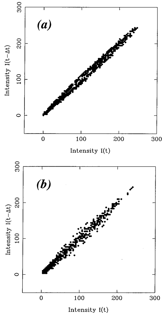
FIG. 7. Relationship plot of the laser dynamics shown in Fig. 6 under repeated drivings. \Delta t is the repetition period of the driving signal, which is 150 \mu\text{s} in our experiment. (a) Relationship plot of the driving signal. (b) Relationship plot of the laser dynamics.
