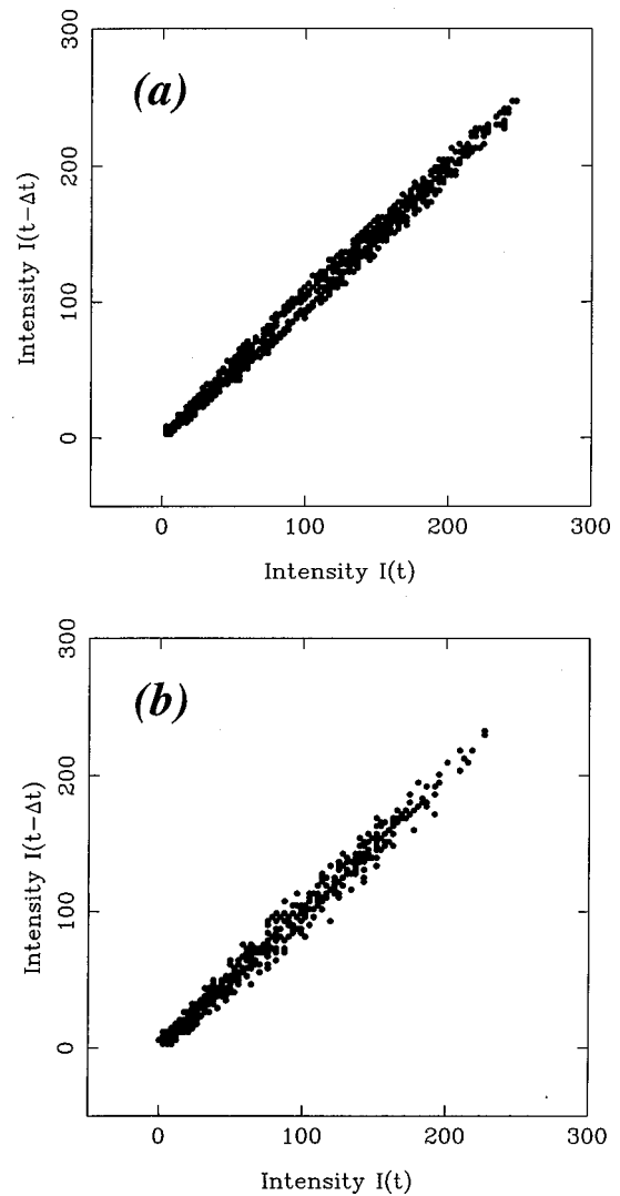
FIG. 5. Relationship plot of the laser dynamics shown in Fig. 4 under repeated drivings. \Delta t is the repetition period of driving signal, which is 150 \mu\text{s} in our experiment. (a) Relationship plot of the driving signal. (b) Relationship plot of the laser dynamics.
