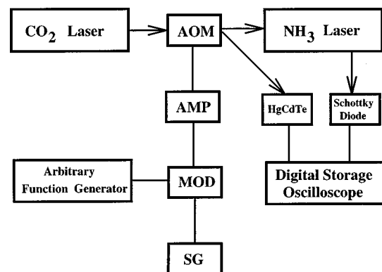
FIG. 1. Schematic block diagram of the experiment setup. SG, signal generator; MOD, modulator; AMP, amplifier; AOM, acousto-optic modulator.
