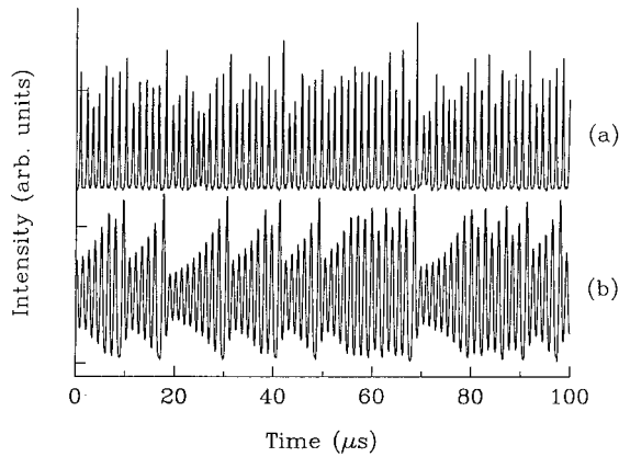
FIG. 4. Chaotic dynamics of the laser under the generalized synchronization of chaos to the driving signal. The average pump laser intensity is 1 \text{ W/cm}^2 and the gas pressure is 19 \mu\text{bar} . Peak-peak pump intensity modulation strength is 23% of the mean pump intensity. (a) Chaotic laser intensity evolution. (b) Evolution of the chaotic driving signal measured.
