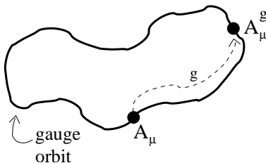
Fig. 1. Illustration of the gauge orbit containing A_\mu and indicating the effect of acting on A_\mu with the gauge transformation g . The action S[A] is constant around the orbit.
