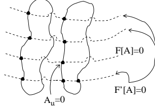
Fig. 2. Ideal, F[A] , and non-ideal, F'[A] , gauge-fixing.
