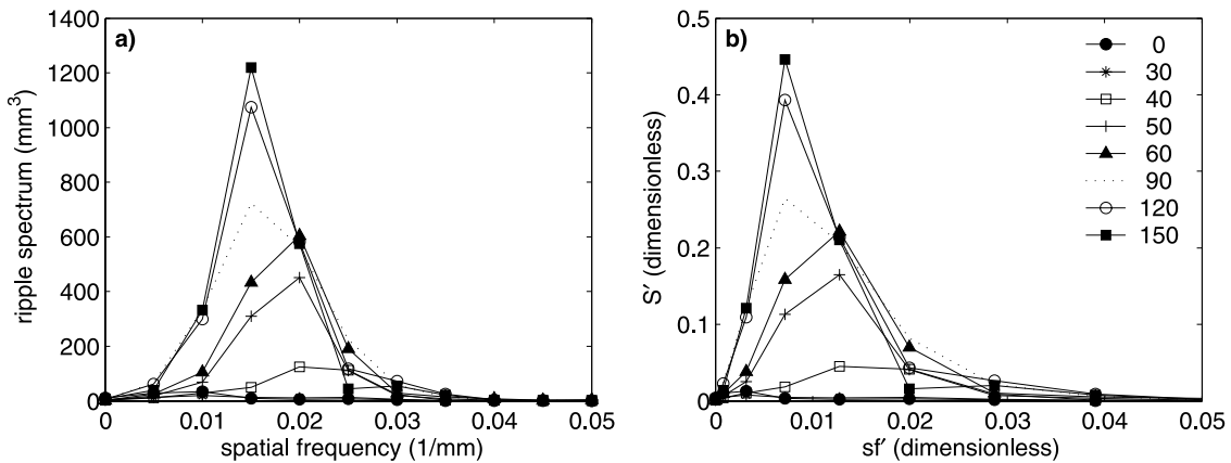
Figure 3. Example plot showing typical ripple spectrum growth with time. (a) Dimensional spectrum calculated from the sediment surface. (b) Ripple spectrum nondimensionalized by the flow and sediment conditions.
