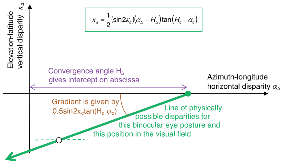
Figure 10. The thick green line shows the line of two-dimensional disparities that are physically possible for real objects, for the given eye posture (specified by convergence H_{\Delta} and gaze azimuth H_c ) and the given visual direction (specified by retinal azimuth \alpha_c and elevation \kappa_c ). The green dot shows where the line terminates on the abscissa. For any given object, where its disparity falls on the green line depends on the distance to the object at this visual direction. The white circle shows one possible distance. Although, for clarity, the green line is shown as having quite a steep gradient, in reality it is very shallow close to the fovea. Thus, it is often a reasonable approximation to assume that the line is flat in the vicinity of the distance one is considering (usually the fixation distance), as indicated by the horizontal green dashed line. This is considered in more detail in the next section.
