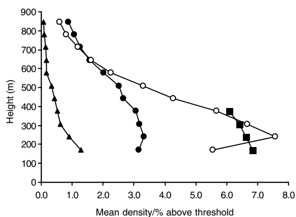
Fig. 10. Vertical distribution of night-flying insects (of mass >10 mg) detected by the Malvern radar in summer 2000. Mean density profiles are shown for June (●), July (▲) and August (○), and 'percentage above threshold' values for August (■).
