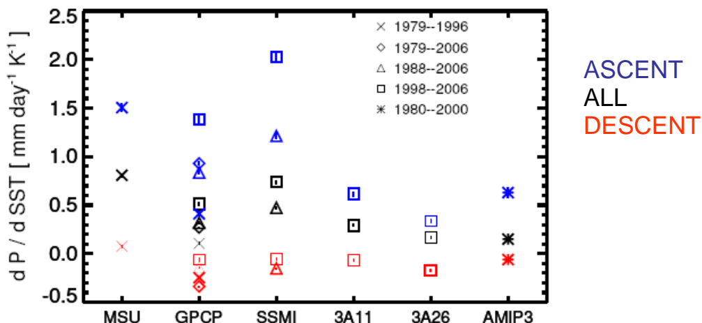
Figure 4: Sensitivity of tropical ocean precipitation to sea surface temperature changes for satellite observations and atmosphere-only climate model simulations and conditioned by positive vertical motion at 500 hPa (descent) and negative vertical motion (ascent).
