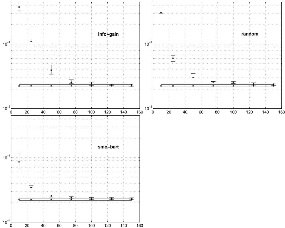
Figure 4.6: Learning curves for sparse GPR on pumadyn-32nm. X-axis: Active set size d . Y-axis: Average squared error.
