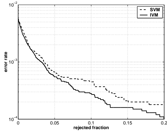
Figure 4.4: Test error rate against increasing rejection rate for the SVM (dashed) and IVM (solid), for the task c = 9 vs. the rest. For SVM, we reject based on “distance” from separating plane, for IVM based on estimates of predictive probabilities. The IVM line runs below the SVM line exhibiting lower classification errors for identical rejection rates.
