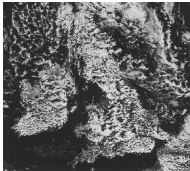
Figure 4. Visible image of the UK from the Modis Aqua satellite at 1245 UTC on 9 May 2005. Courtesy of NASA Goddard Space Flight Center.
