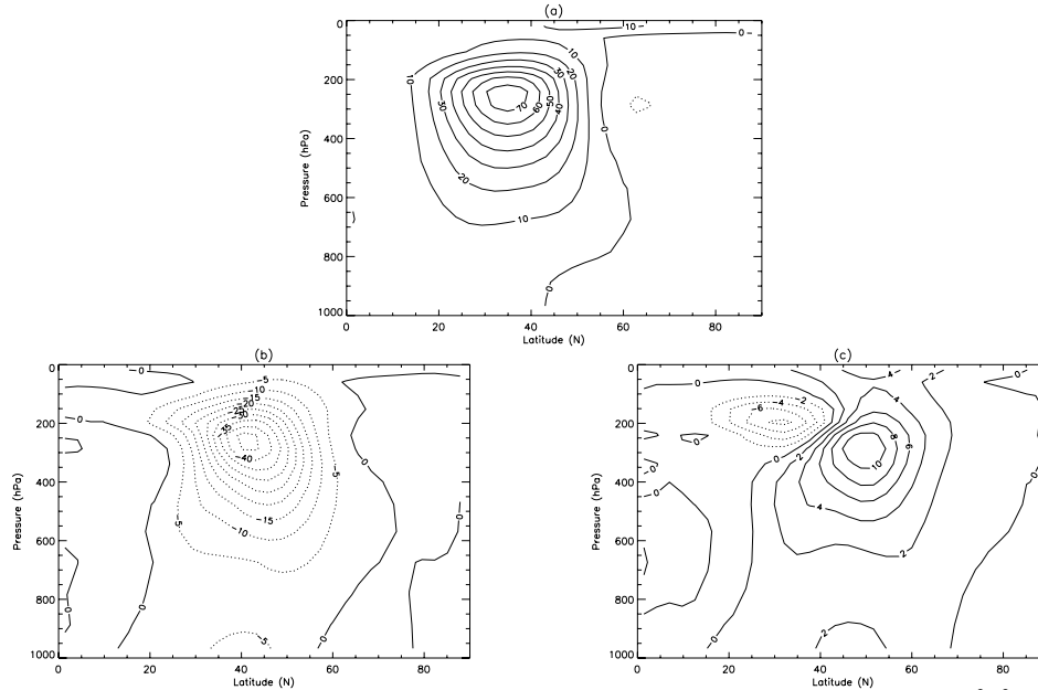
Figure 4 Poleward flux of westerly momentum by the zonally asymmetric eddies [ u'v' ] ( \text{m}^2\text{s}^{-2} ) for (a) the control run C; (b) the U5 - C anomaly and (c) the E5 - C anomaly. Average of 2 hemispheres.
