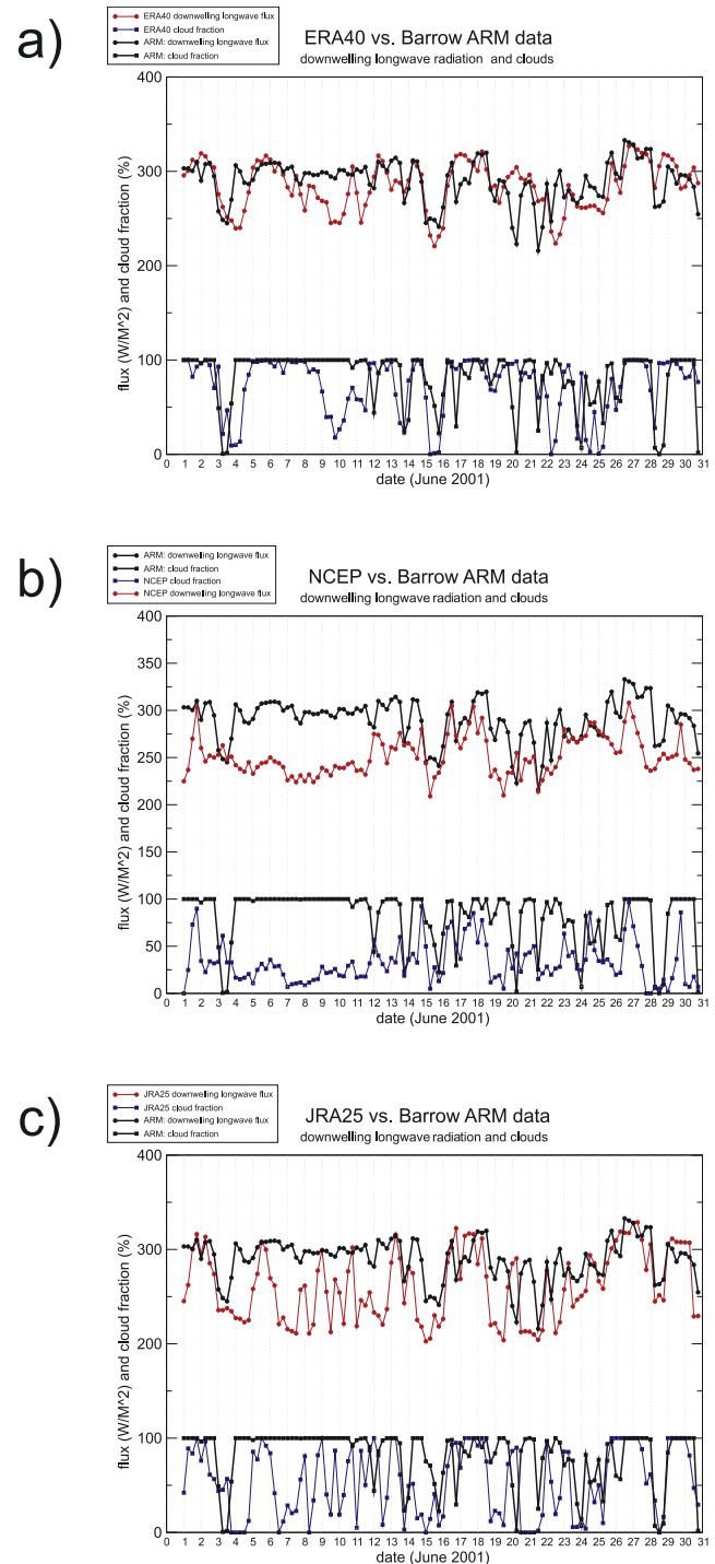
Figure 12. As in Figure 11, but for downwelling longwave radiation.
