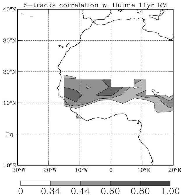
FIG. 9. Correlation map of 11-yr running mean July–October tracks from the southern storm-track area and Hulme precipitation. Shading starts at 95% significance using a Student's t test.
