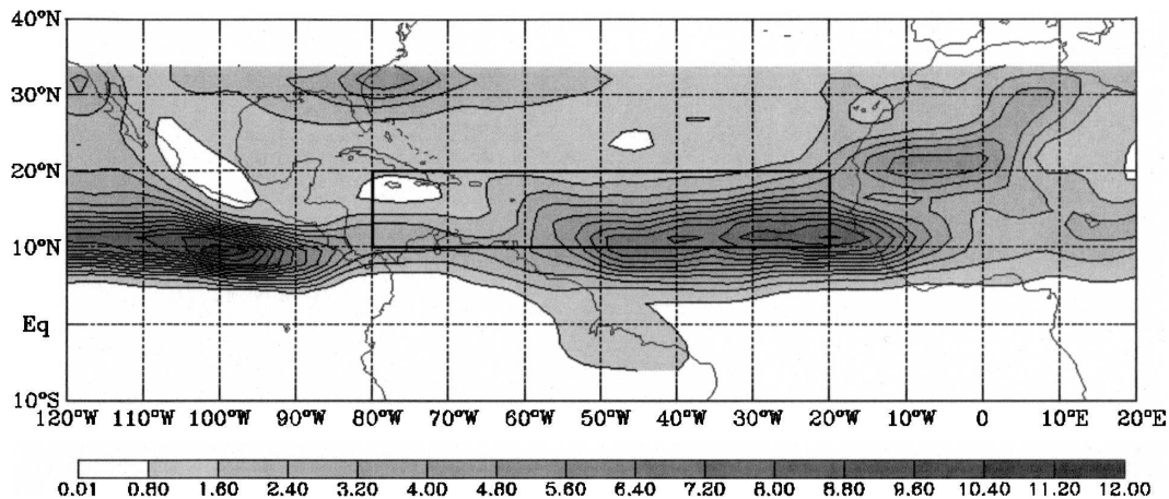
FIG. 1. Track density [scaled to number density per unit area [with unit area equivalent to a 5^\circ radius spherical cap ( \sim 10^6 km ^2 )] per month of all storm tracks over the mapped area for the months of May–November and years 1958–2002. Contour intervals (CIs) every 0.8, starting at 0.01. Also shown is the outline of the MDR and latitude–longitude lines every 10^\circ .
