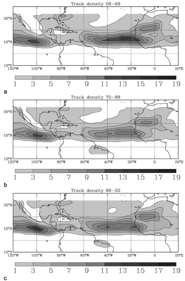
FIG. 12. Mean track density [scaled to number density per unit area [with unit area equivalent to a 5^\circ radius spherical cap ( \sim 10^6 km 2 )] per season (JASO) for (a) the active period from 1958 to 1969, (b) the inactive period from 1970 to 1988, and (c) the active period from 1989 to 2002.
