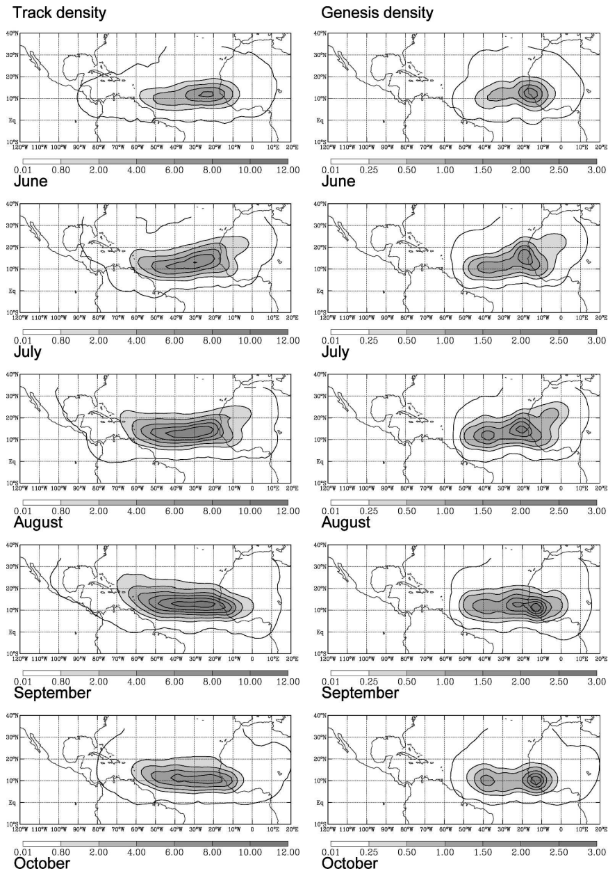
FIG. 4. Track density and genesis density [scaled to number density per unit area [with unit area equivalent to a 5^\circ radius spherical cap ( \sim 10^6 km ^2 )] per month], shown for the months of June–October, from top to bottom. The statistics maps are produced using all tracks (1958–2002) that pass through the eastern half of the MDR ( 10^\circ – 20^\circ N, 20^\circ – 50^\circ W). Latitudes and longitudes are shown for every 10^\circ .
