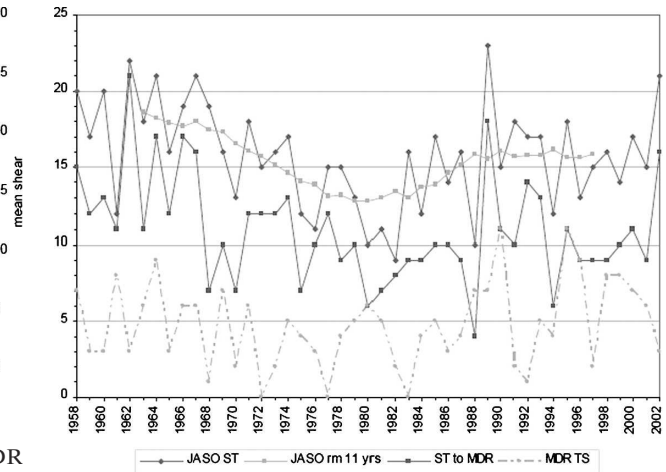
FIG. 8. Number of storms at 850 hPa counted along the ST (thick solid) and 11-yr running mean value (RM; gray) for July–October 1958–2002. Also shown is the number of storms proceeding to the MDR over the tropical Atlantic (thin solid) and the number of MDR tropical storms from the NHC best-track dataset (dash-dot-dot).
