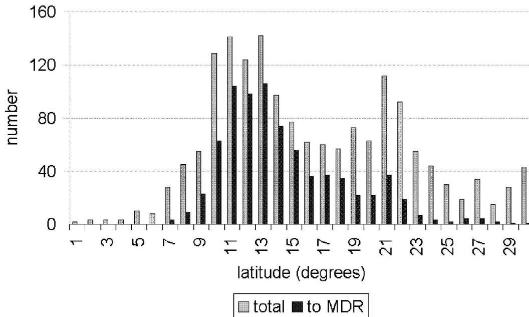
FIG. 3. Number of storm tracks during May–November, from 1958 to 2002, found within longitude of 10° to 20°W and number of storm tracks that further continue to the MDR (light and dark gray, respectively) vs latitude.
