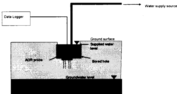
Fig.1 Field setup to determine the in-situ effective porosity
