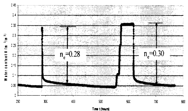
Fig.7 Water content versus time for river sand (vertical ADR probe in bigger diameter column)
