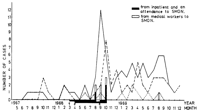
Fig. 5 Number of patients entering hospital (solid line), those of leaving hospital (dotted line), those in hospital (chain line), intra-hospital occurrence of non-SMON patients (solid column) and medical workers (open column) and arrow shows the date entering hospital of non-SMON patients.
