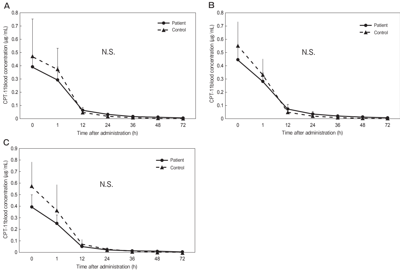
Fig. 3 CPT-11 blood concentration curve after administration of CPT-11 at 50\text{mg/m}^2 (A), 60\text{mg/m}^2 (B) and 70\text{mg/m}^2 (C) in dialysis patients and controls.
