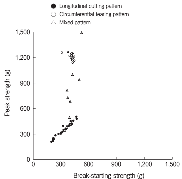
Fig. 6 Relation between peak strength (suture retention strength) and break-starting strength.
