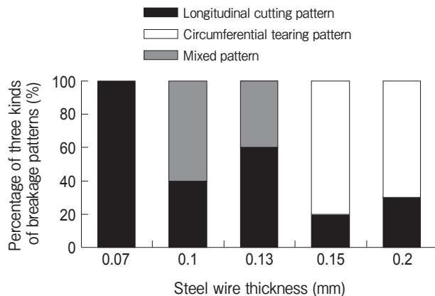
Fig. 4 Percentage of 3 kinds of breakage patterns in relation to thickness of steel wire thickness.
