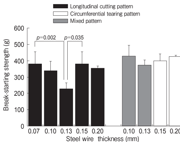
Fig. 9 Average break-starting strength of 3 kinds of breakage patterns in relation to steel wire thicknesses. Error bars represent one standard deviation of the mean.
