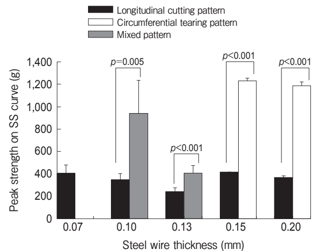
Fig. 5 Average peak strength (suture retention strength) of 3 kinds of breakage patterns in relation to steel wire thickness. Error bars represent one standard deviation of the mean.
