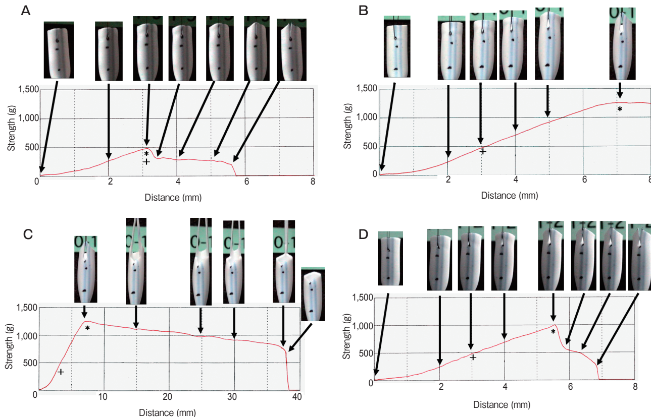
Fig. 2 Stress-strain curve and photographs of the breakage of ePTFE graft in the longitudinal cutting pattern (A), the circumferential tearing pattern from zero point to the point of peak strength (B) and from the zero point to the end point of the breakage (C), and the mixed pattern (D). *, Peak strength (suture retention strength); +, Break-starting strength.
