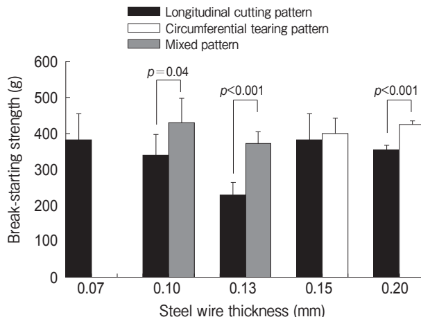
Fig. 8 Average break-starting strength of 3 kinds of breakage patterns in relation to steel wire thicknesses. Error bars represent one standard deviation of the mean.
