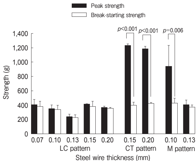
Fig. 7 Average peak strength (suture retention strength) and break-starting strength in 3 kinds of breakage patterns in relation to steel wire thicknesses. Error bars represent one standard deviation of the mean. LC pattern, longitudinal cutting pattern; CT pattern, circumferential tearing pattern; M pattern, mixed pattern.
