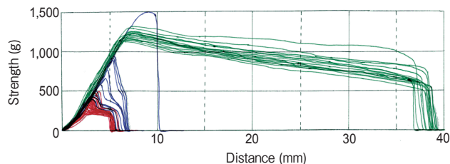
Fig. 3 Typical stress-strain curves of longitudinal cutting pattern (red), mixed pattern (blue) and circumferential tearing pattern (green) were shown on the same coordinate axes.
