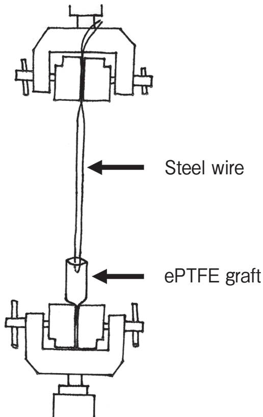
Fig. 1 Schema of the testing method of suture retention strength.
