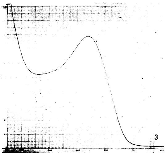
Fig. 3 Absorbancy of the peptide of tumor ribosomal digest. Maximum absorbance of the peptide (Peak I in Fig. 2) was observed at 267 m \mu .
