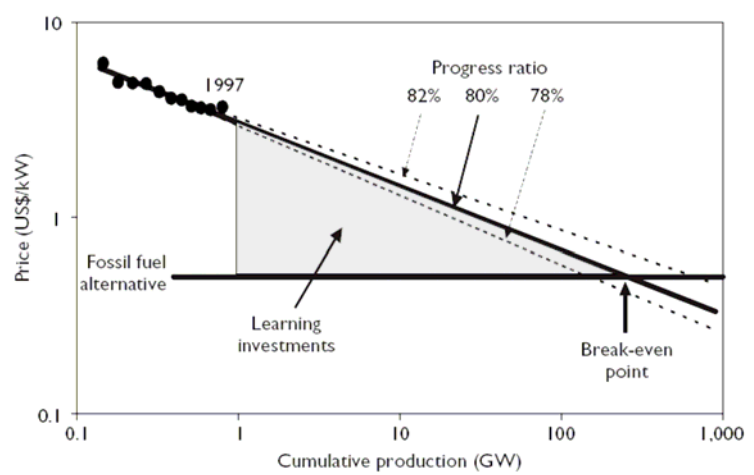
Figure 3 Making Photovoltaics Break-Even (IEA 2000, p15).
